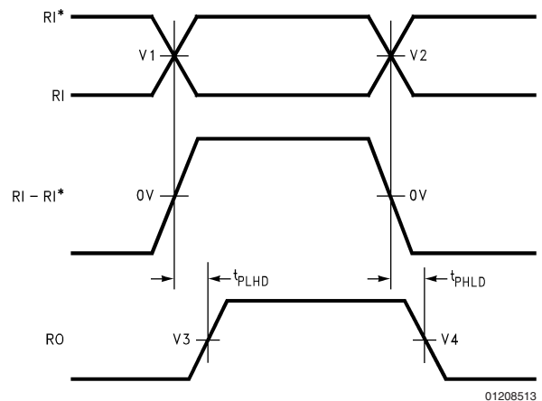
FIGURE 8. Propagation Delay Waveforms for Circuit 3 (see Figure 7)
