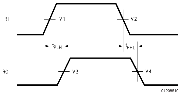
FIGURE 6. Propagation Delay Waveforms for Circuit 1 and Circuit 2 (See Figure 5)
