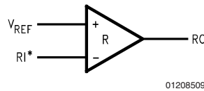
FIGURE 5. Circuits for Measuring Single-Ended Propagation Delays (See Figure 6)
