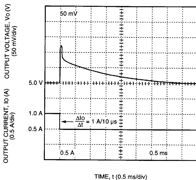
Figure 4. DC025 Dual-Output-Series Typical 5 V Output Voltage Response to a Step Load Change from 50% to 25% of I_{o, \max} at V_i = V_{i, \text{nom}} and T_c = 25^\circ\text{C}
