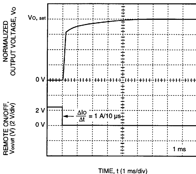
Figure 10. DC025 Dual-Output-Series Typical Output Voltage Rise Time with Remote On/Off at V_i = V_{i,nom} , I_o = 0.8 (I_{o,max}) , and T_c = 25\text{ }^{\circ}\text{C}
