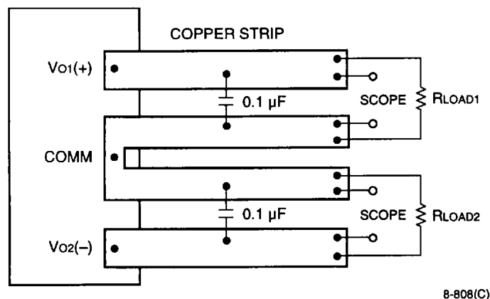
A. Pinout A (DC025AJ-M, BK-M, CL-M) Configuration
