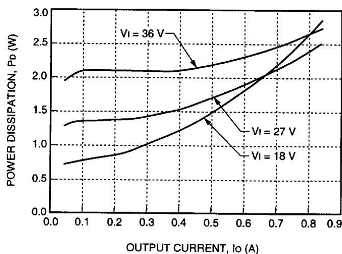
Figure 19. 15 V Output Power Dissipation vs. Output Current
