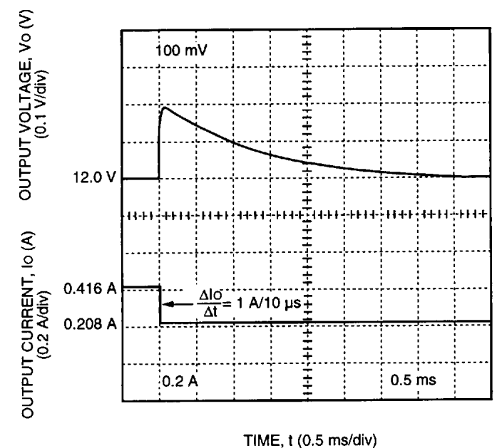
Figure 5. DC025 Dual-Output-Series Typical 12 V Output Voltage Response to a Step Load Change from 50% to 25% of I_{o,max} at V_i = V_{i,nom} and T_c = 25^\circ\text{C}
