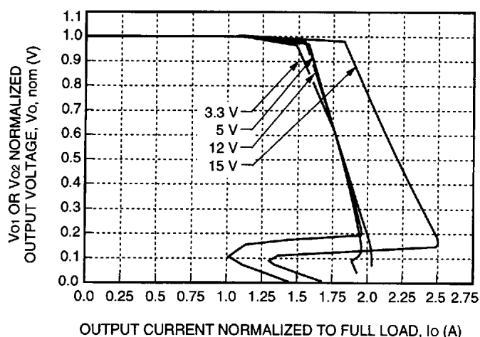
Figure 2. DC025 Dual-Output-Series Normalized Output Current vs. Normalized Output Voltage at V_i = 28\text{ V} and T_c = 25^\circ\text{C}
