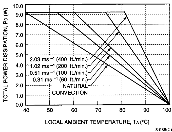
Figure 20. Total Power Dissipation vs. Local Ambient Temperature and Air Velocity
