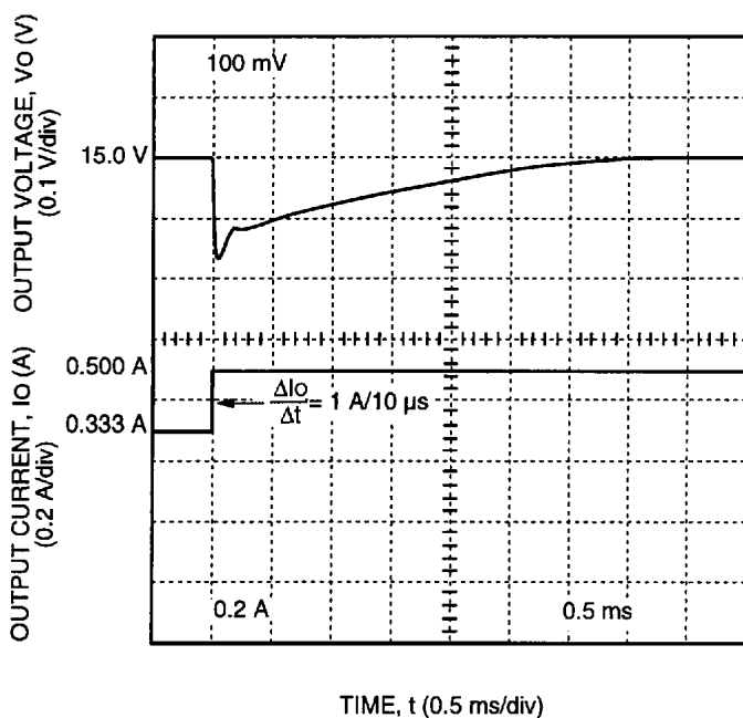
Figure 9. DC025 Dual-Output-Series Typical 15 V Output Voltage Response to a Step Load Change from 50% to 75% of I_{o,max} at V_i = V_{i,nom} and T_c = 25\text{ }^{\circ}\text{C}
