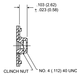
E-Clinch Nut
