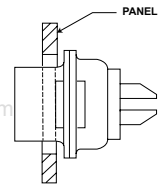
Rear mounting of float mount shell (Y-Code)
