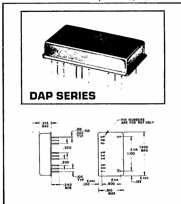
HERMETIC PACKAGE
