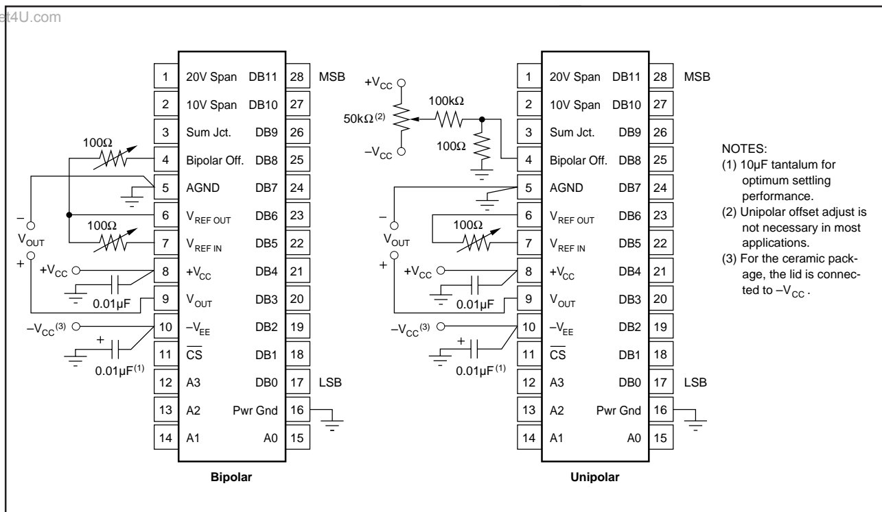
FIGURE 5. Power Supply, Gain and Offset Connections.
