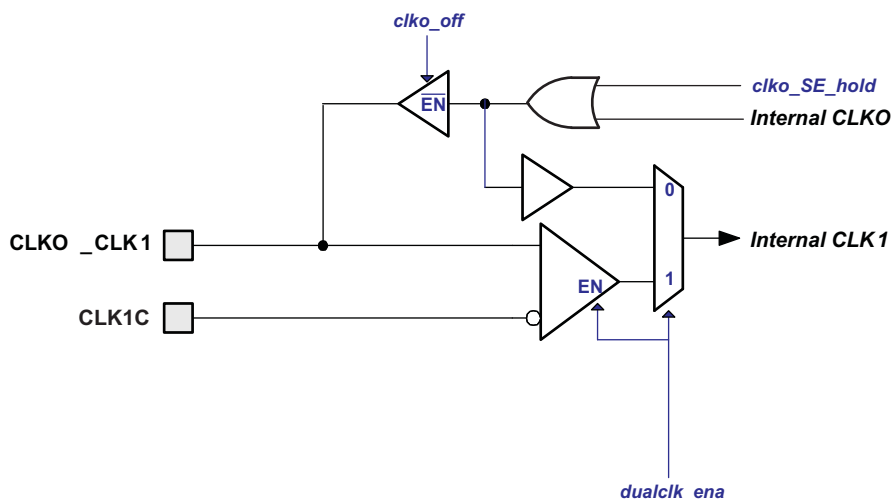
Figure 35. CLKO_CLK1 and CLK1C Pins Control
