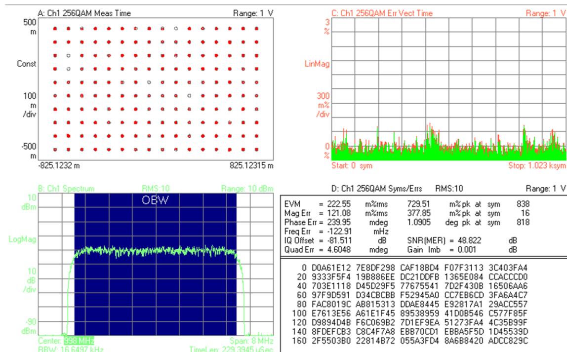
Figure 147. Unequalized MER of 6 MHz Single Carrier at 998 MHz
