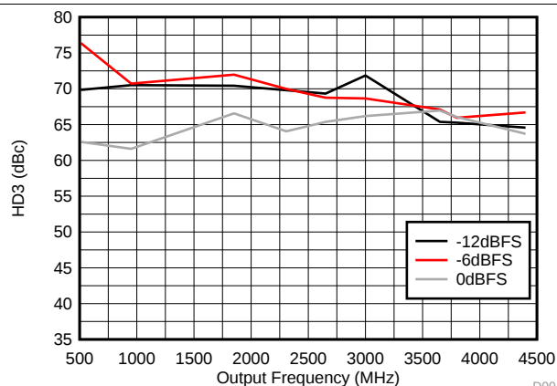
D004 DAC38RF83/93/85
