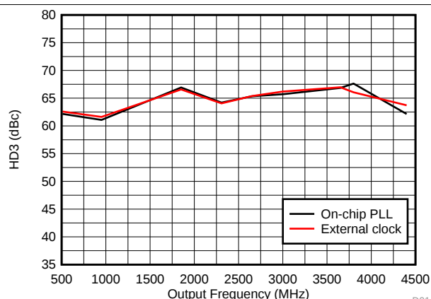
D014 DAC38RF83/93/85
