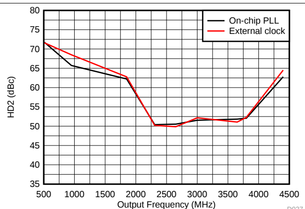
D027 DAC38RF80/90/84
