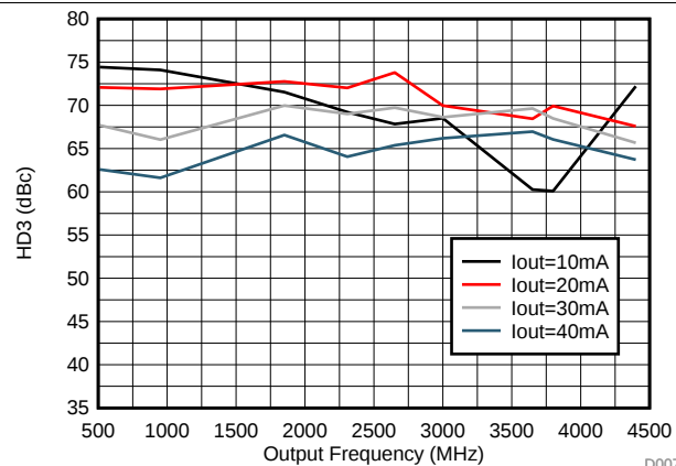
D007 DAC38RF80/90/84
