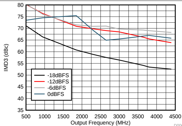
D006 DAC38RF83/93/85
