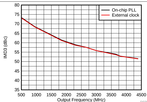
D030 DAC38RF80/90/84
