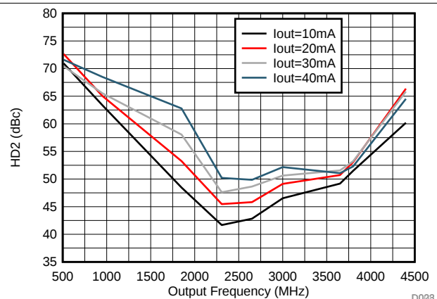
D028 DAC38RF80/90/84
