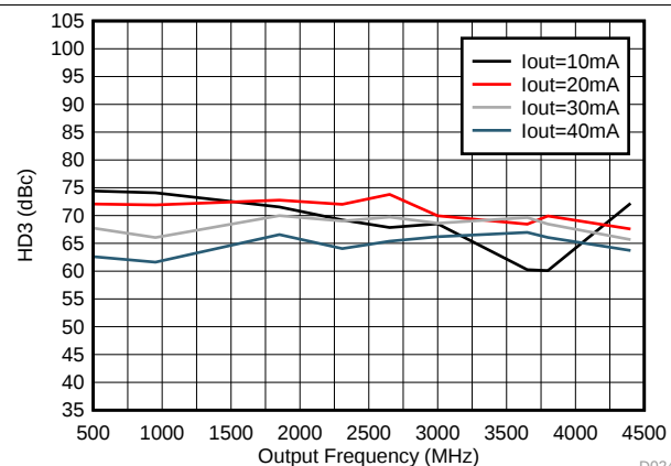
D024 DAC38RF83/93/85
