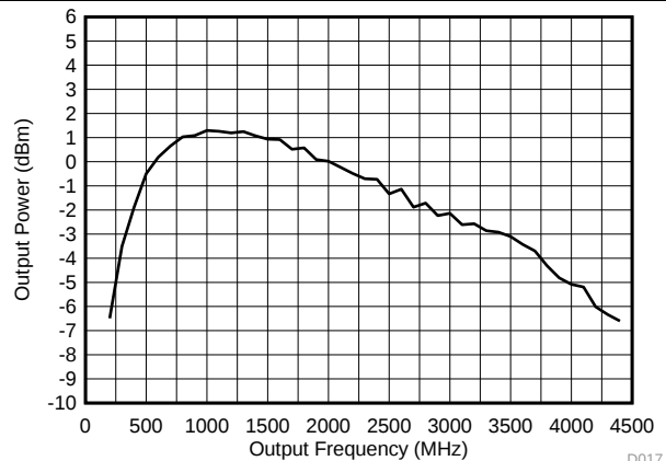
DAC38RF80/90/84
