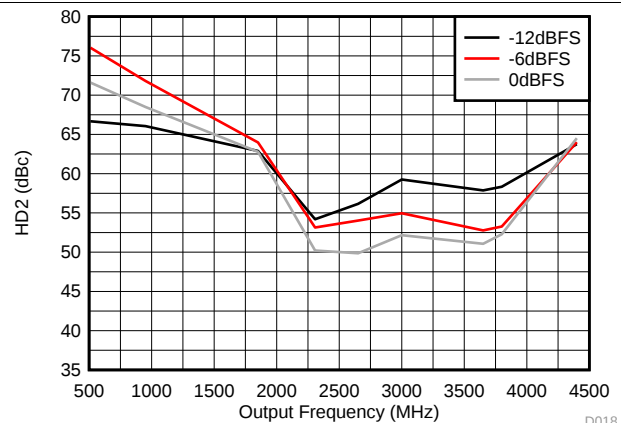
D018 DAC38RF80/90/84
