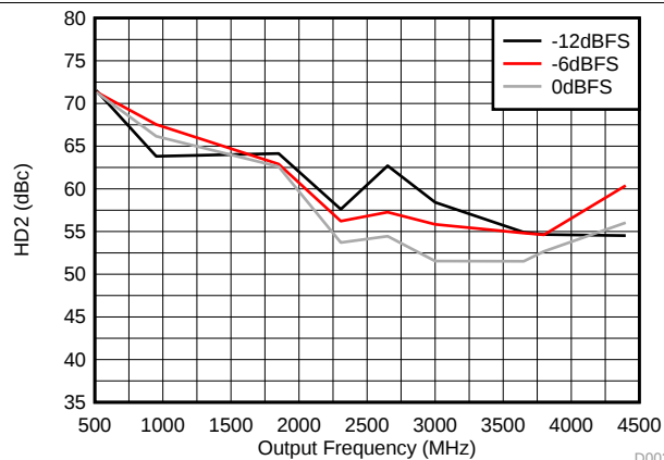
D002 DAC38RF83/93/85
