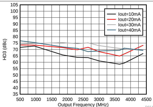
D014 DAC38RF80/90/84
