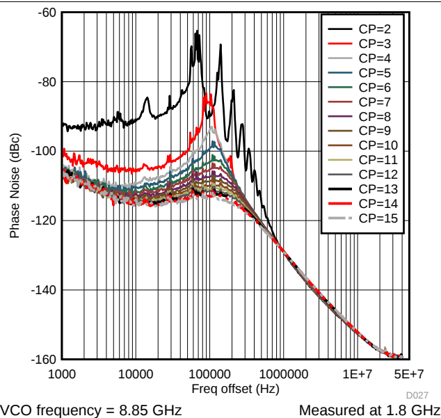
Figure 41. VCO1 Phase Noise vs Offset Frequency Over Charge pump current
