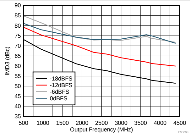
D006 DAC38RF80/90/84
