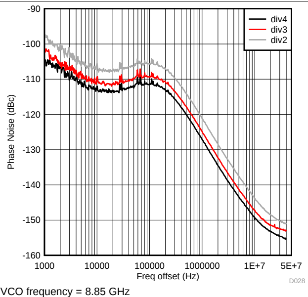
Figure 42. VCO1 Output Clock Phase Noise vs Offset frequency Over Divider Ratio
