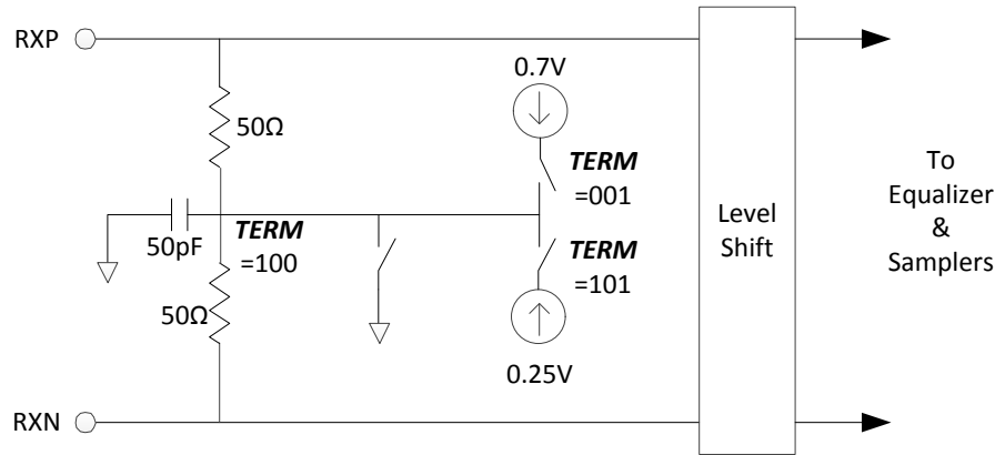
Figure 51. Serial Lane Input Termination
