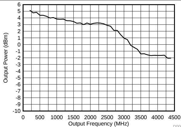
Transformer loss not de-embedded DAC38RF83/93/85
