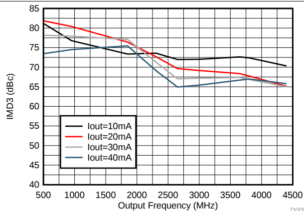
D009 DAC38RF83/93/85
