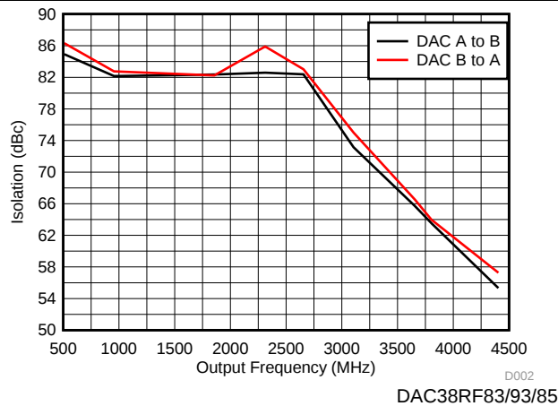
Figure 39. Isolation vs Output Frequency
