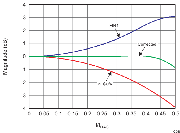
Figure 67. Composite Magnitude Spectrum for INVSINC
