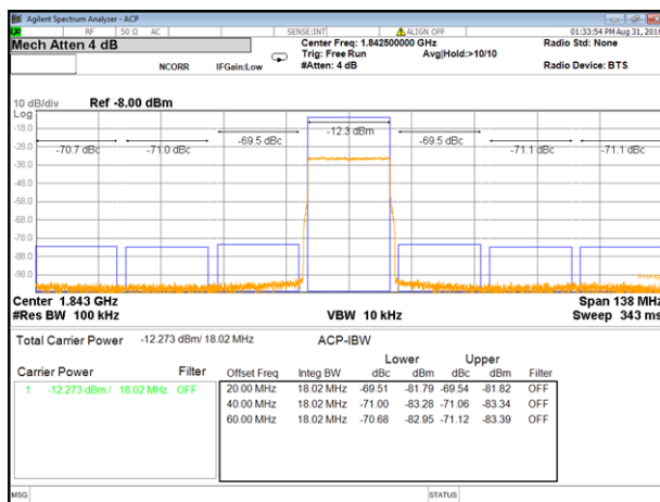
Figure 170. Dual band ACPR Performance in Downlink Band 3 with On-chip PLL
