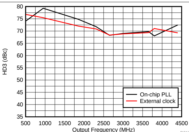
D015 DAC38RF80/90/84
