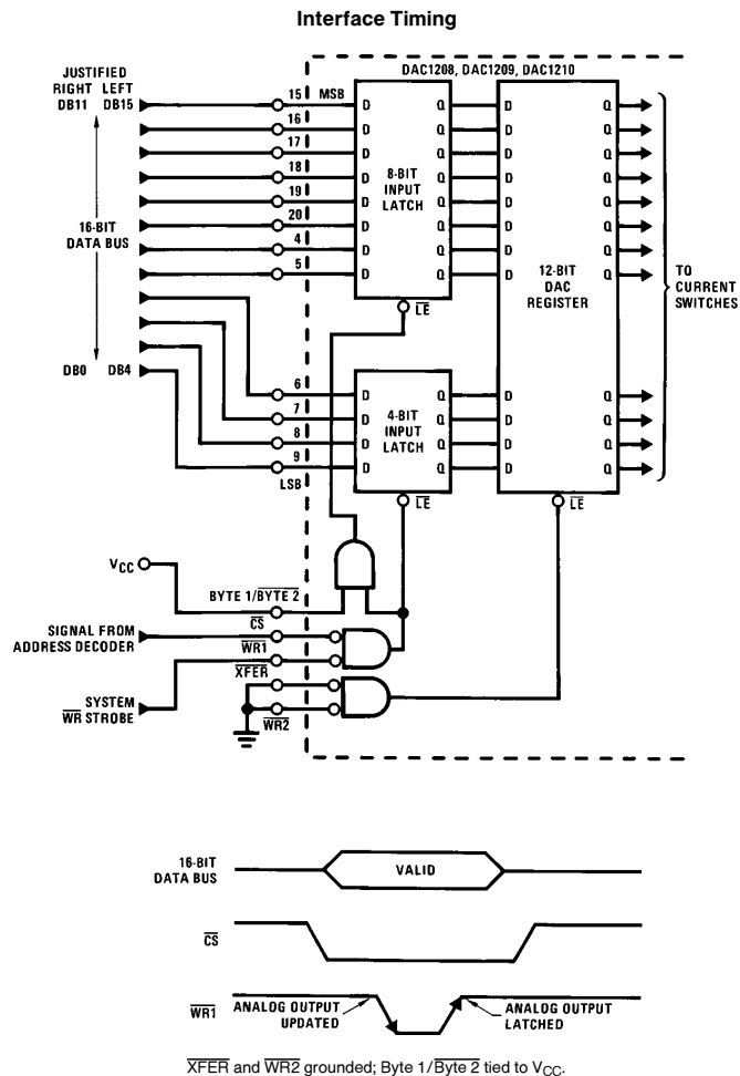
FIGURE 4. 16-Bit Data Bus Interface for the DAC1208 Series
