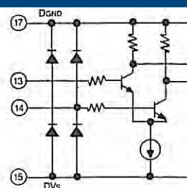
Figure 1. Clock Inputs
