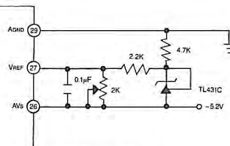
Figure 4. Voltage Reference
