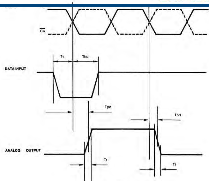
Figure 6. Timing Diagram
