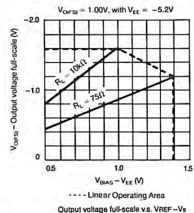
Figure 9. Output Voltage Full-Scale vs VREF - Vs
