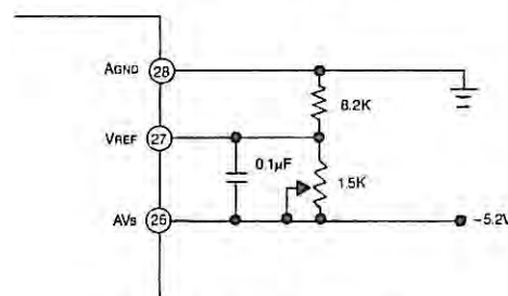
Figure 3. Voltage Reference
