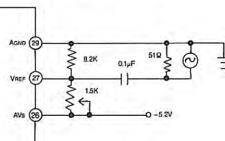
Figure 5. Multiple Circuits
