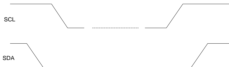
Figure 33: I 2 C START and STOP Conditions
