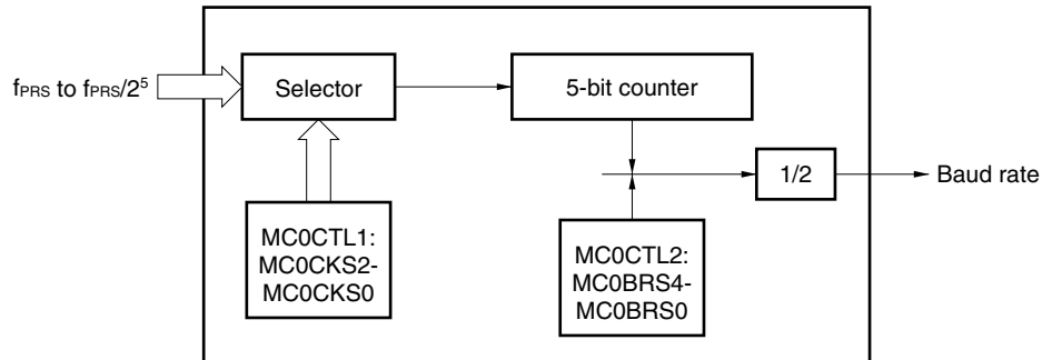
Figure 19-2. Block Diagram of Baud Rate Generator
