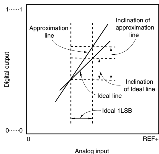
Figure 13-18. Gain Error
