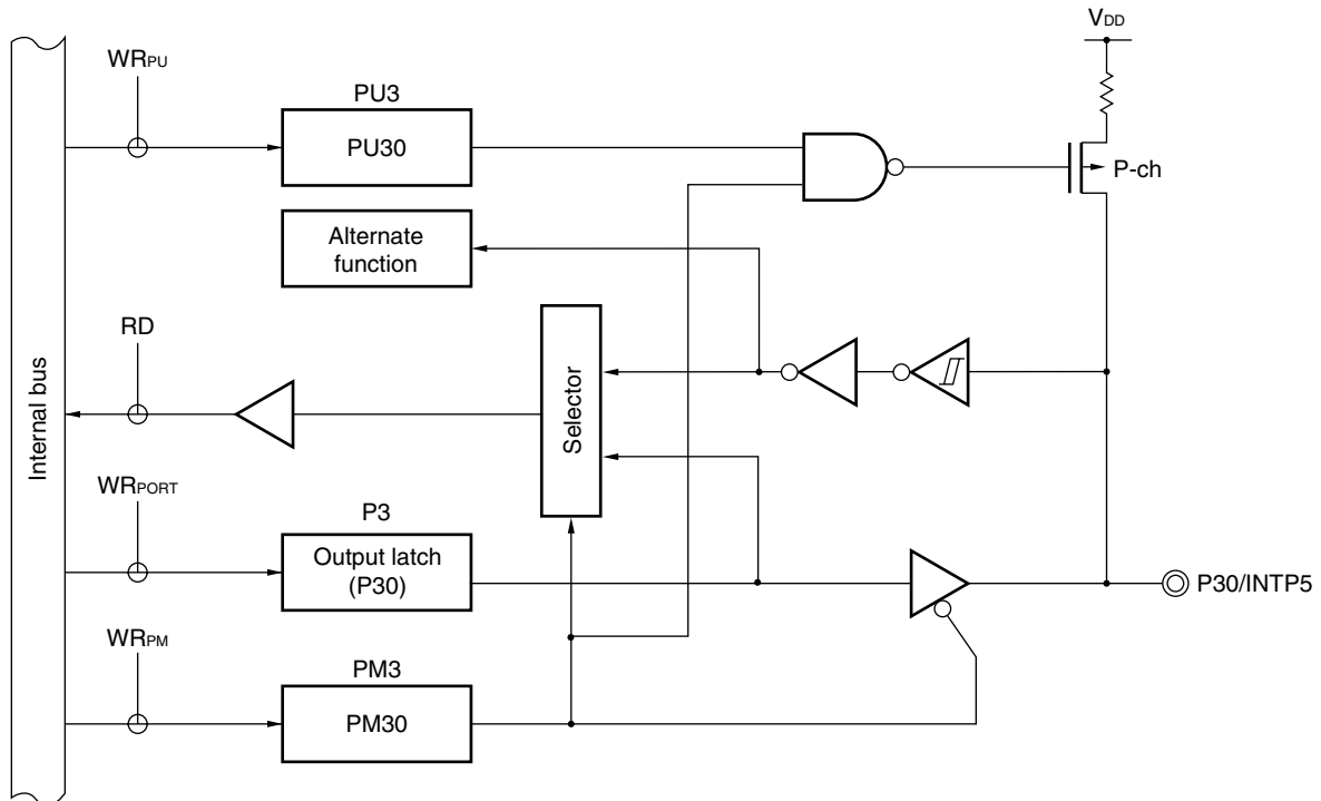
Figure 4-9. Block Diagram of P30
