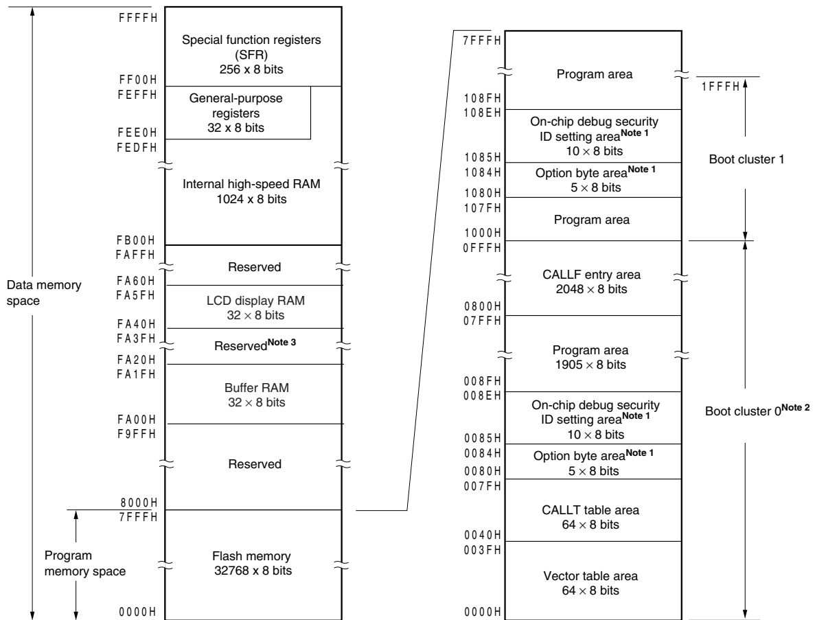
Figure 3-6. Memory Map ( \mu PD78F0493)
