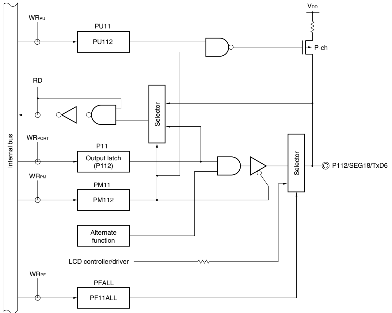
Figure 4-19. Block Diagram of P12
