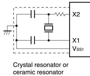
(a) Crystal and ceramic oscillation
