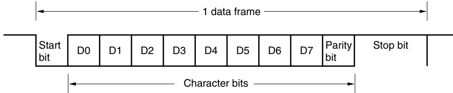
Figure 14-8. Example of Transmit/Receive Data Format in Asynchronous Serial Interface
