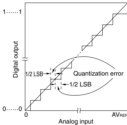
Figure 13-12. Quantization Error
