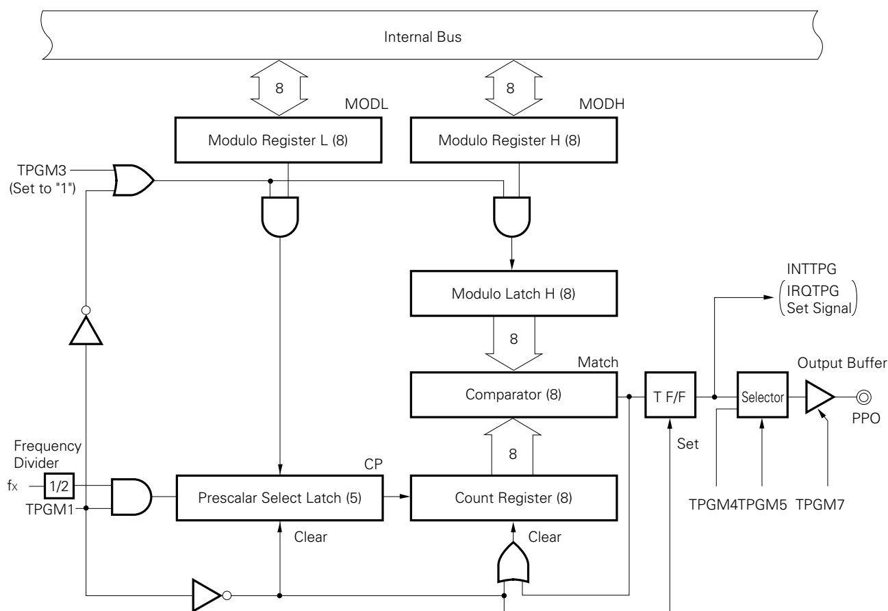
Fig. 5-5 Block Diagram of Timer/Pulse Generator (Timer Mode)
