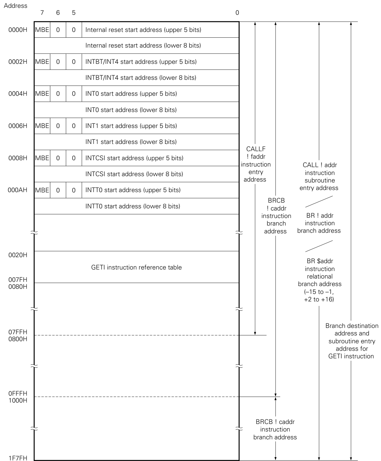
Fig. 4-3 Program Memory Map ( \mu PD75008)
