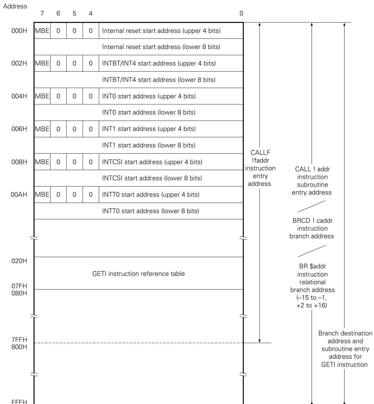
Fig. 4-1 Program Memory Map ( \mu PD75004)
