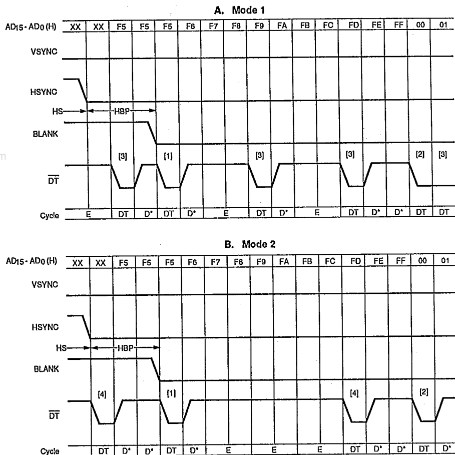
Figure 5. \overline{DT} Signal Output, Mode 1 and Mode 2
