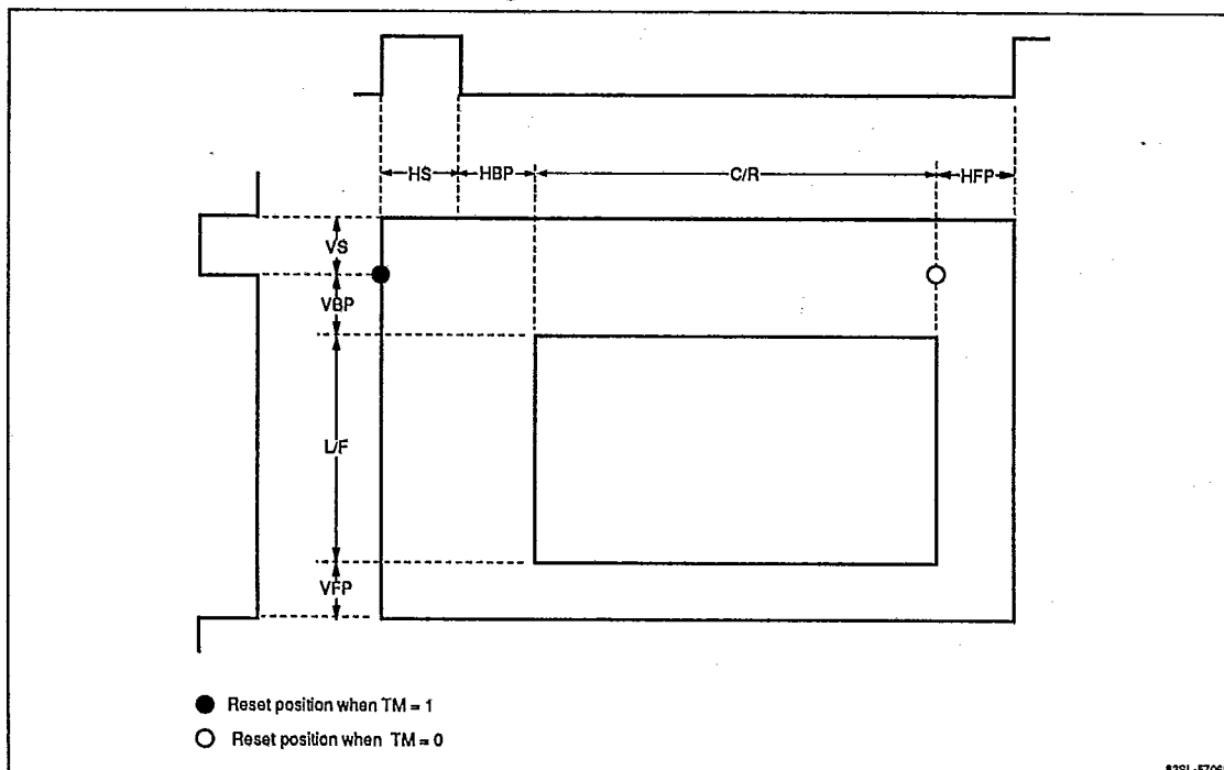
Figure 2. Horizontal Counter Reset Timing
