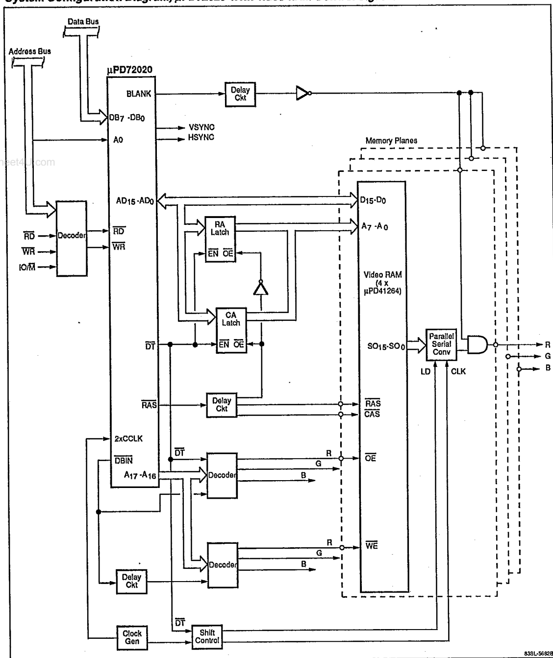
System Configuration Diagram; μPD72020 With Video RAM Control Signal \overline{DT}
