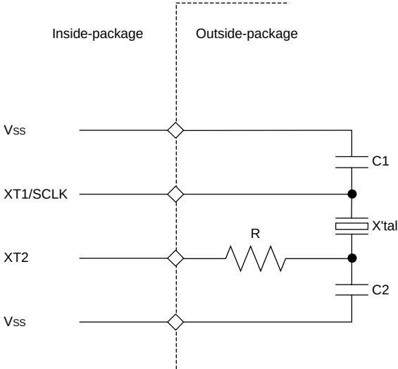
Figure 2-3. X'tal Connection
