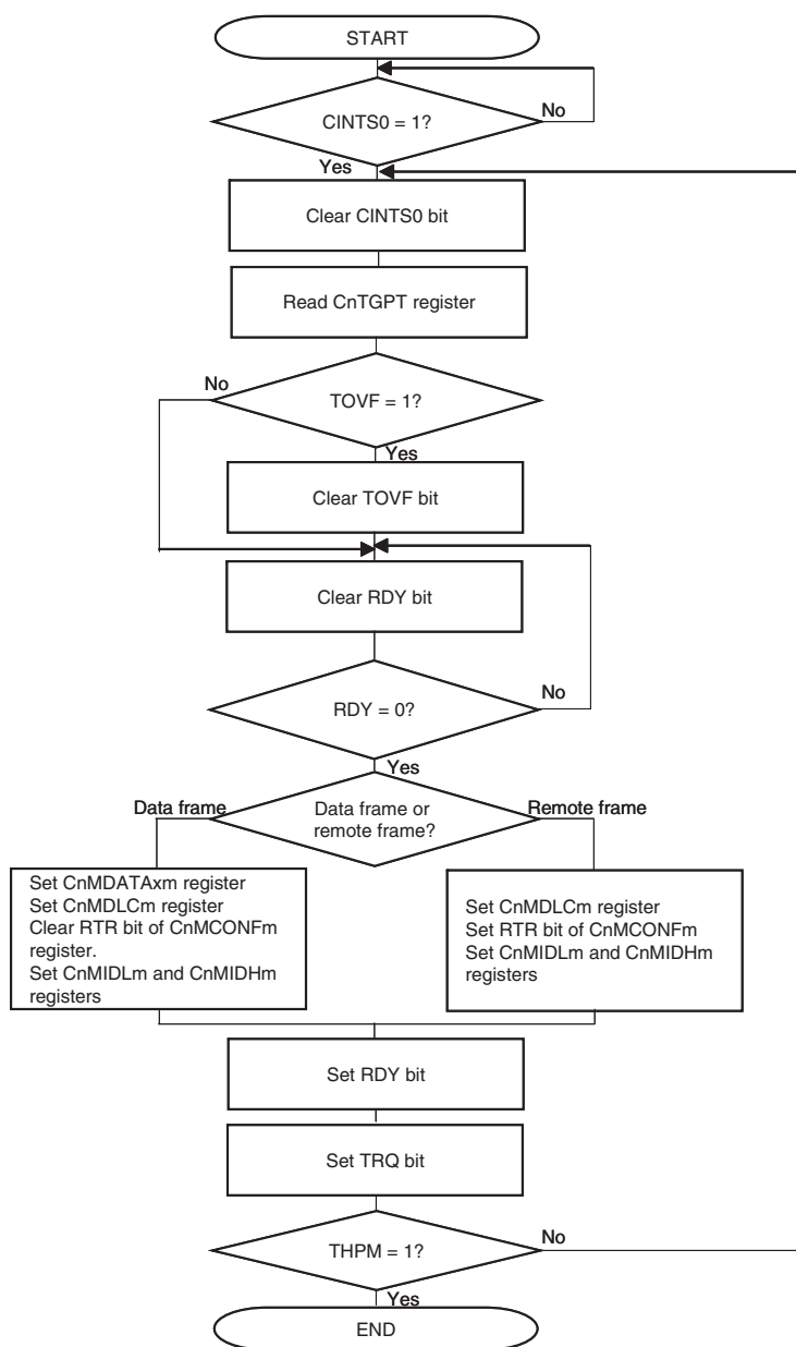
Figure 20-44 Transmission via software polling
