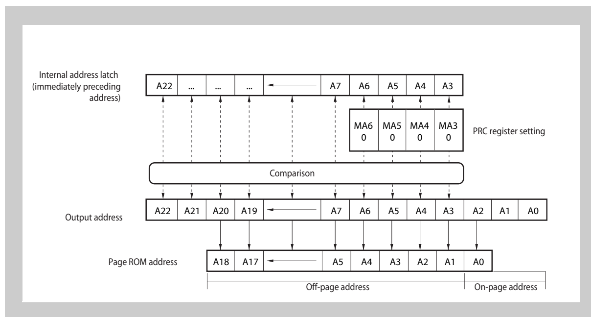
Figure 7-7 16-Mbit page ROM (512 k x 32 bits), page size 2 x 32 bit
