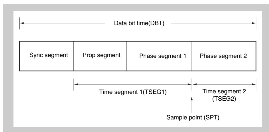
Figure 20-18 Segment setting
