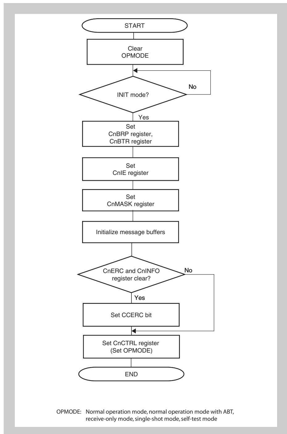
Figure 20-36 Re-initialization
