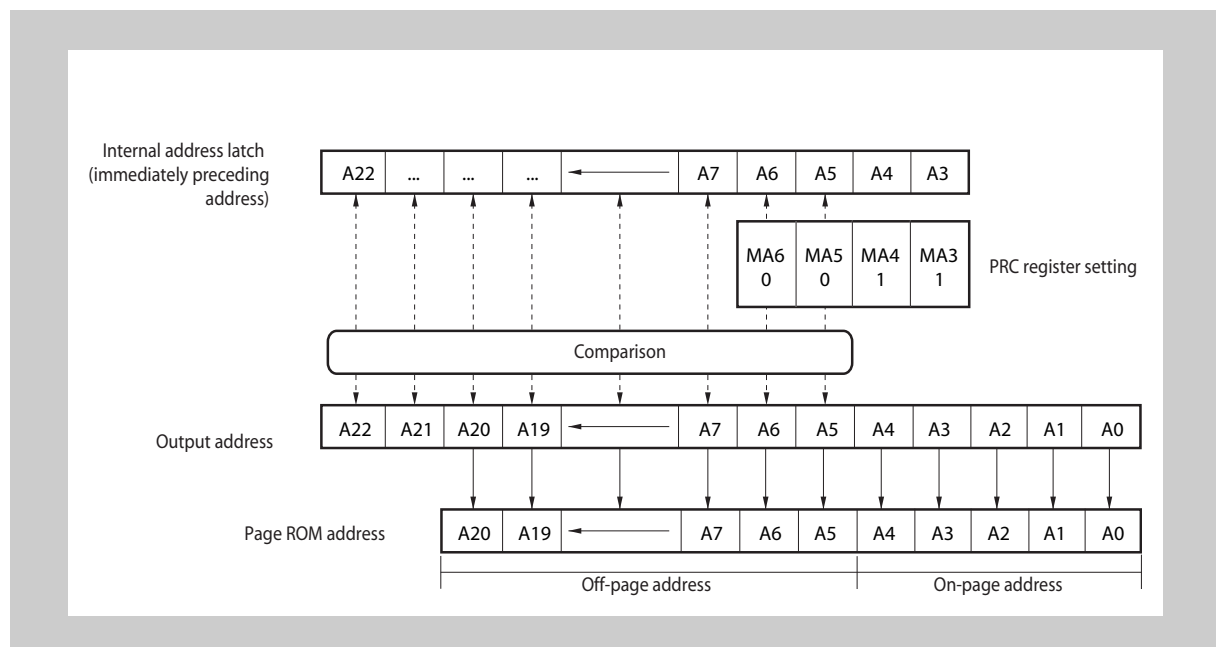
Figure 7-5 16-Mbit page ROM (2 M x 8 bits), page size 32 x 8 bit
