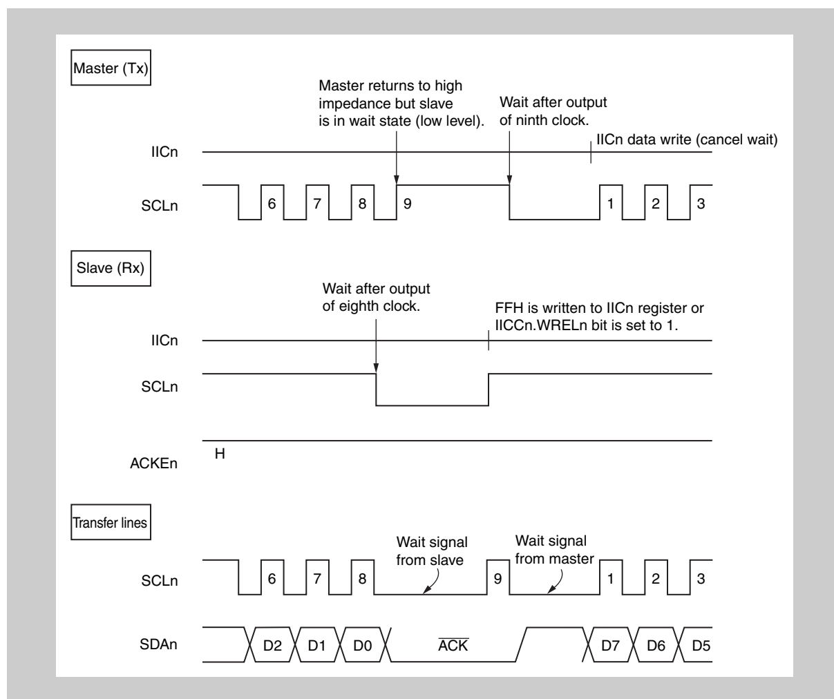
Figure 19-12 Wait signal (1/2)
