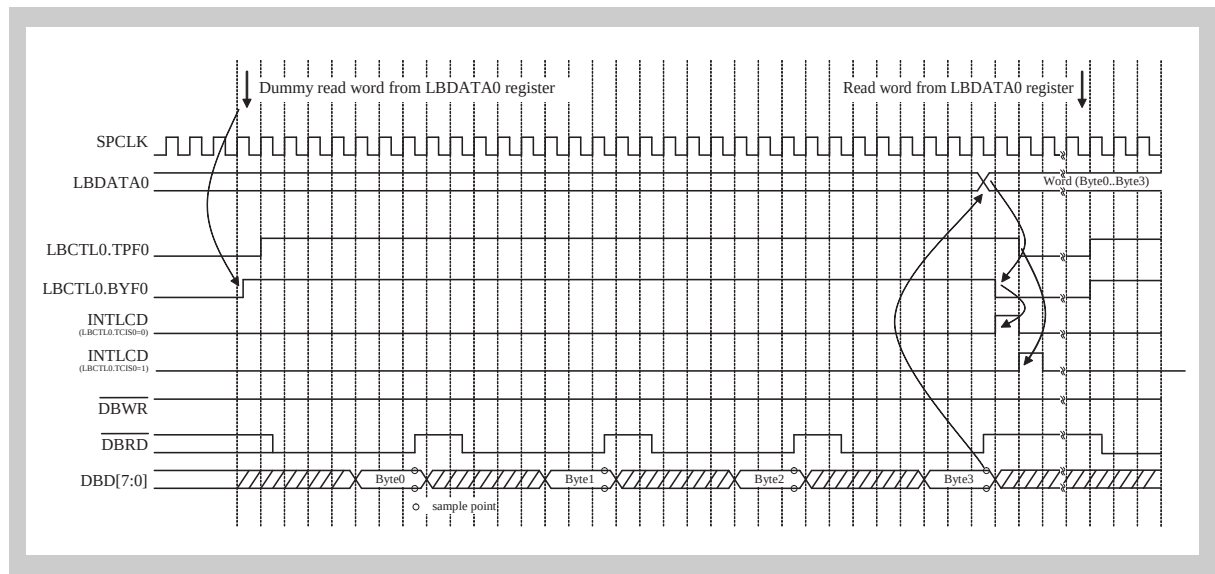
Figure 24-6 Timing (mod80: LBTCTL0.IMD0 = 0): read word, LBWST0.WST0 = 5, LBCYC0.CYC0 = 8, LBCTL0.TCIS0 = 0 and 1
