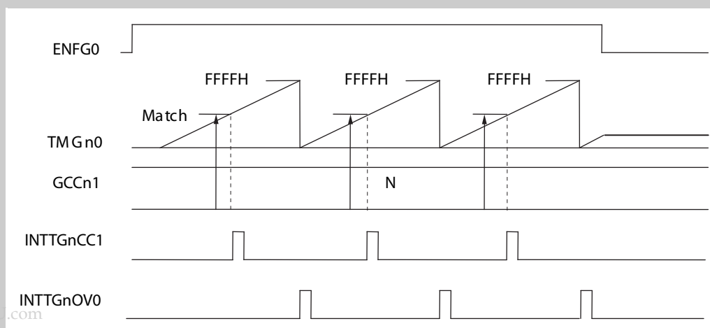
Figure 13-6 Timing of compare mode (free run)
