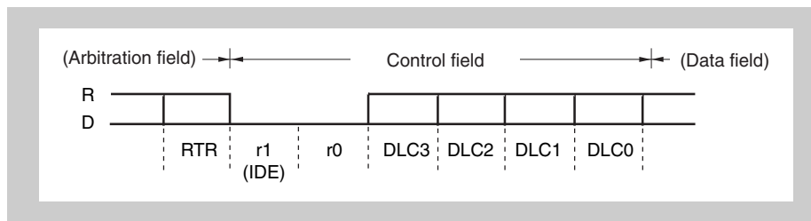
Figure 20-8 Control field
