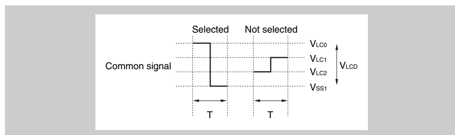
Figure 23-4 Selection level and non-selection level of common signals
