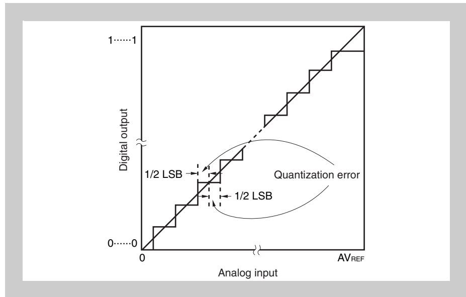
Figure 21-11 Quantization error
