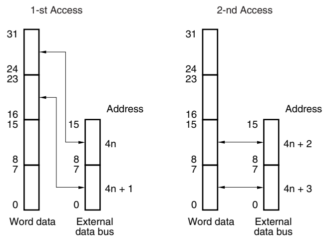
Figure 7-41 Access to address 4n
