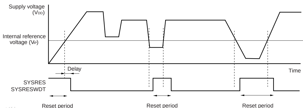
Figure 27-2 Timing of internal reset signal generation by Power-On-Clear circuit
