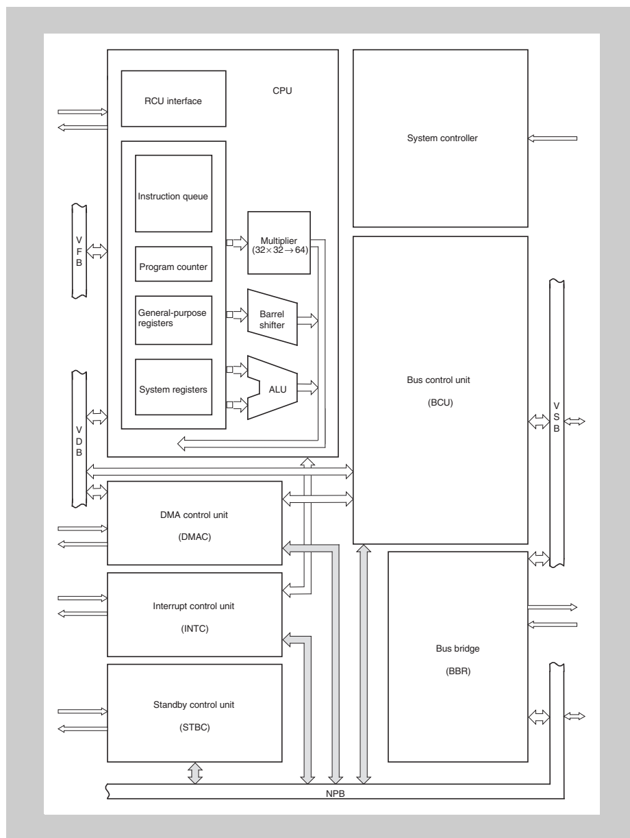
Figure 3-1 CPU system
