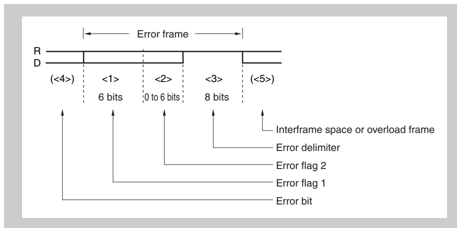
Figure 20-15 Error frame
