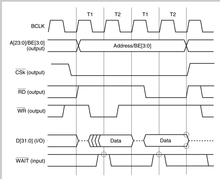
Figure 7-16 Write-read operation
