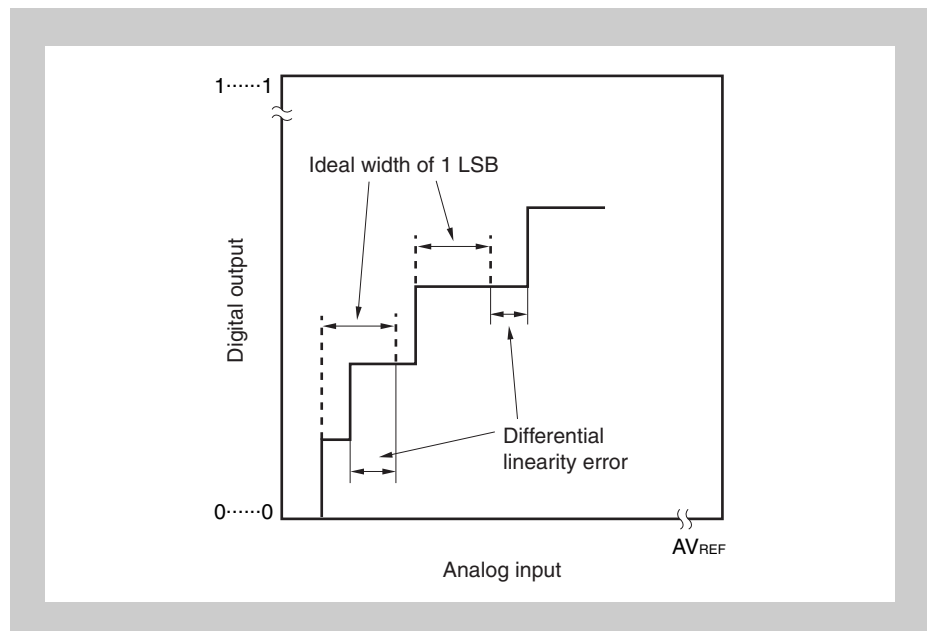
Figure 21-14 Differential linearity error
