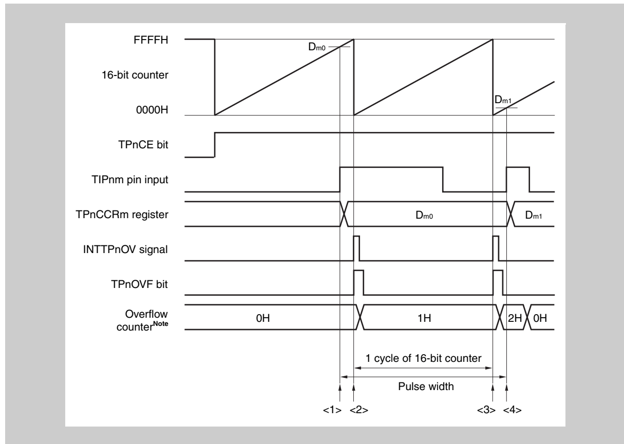
Figure 11-36 Example when capture trigger interval is long
