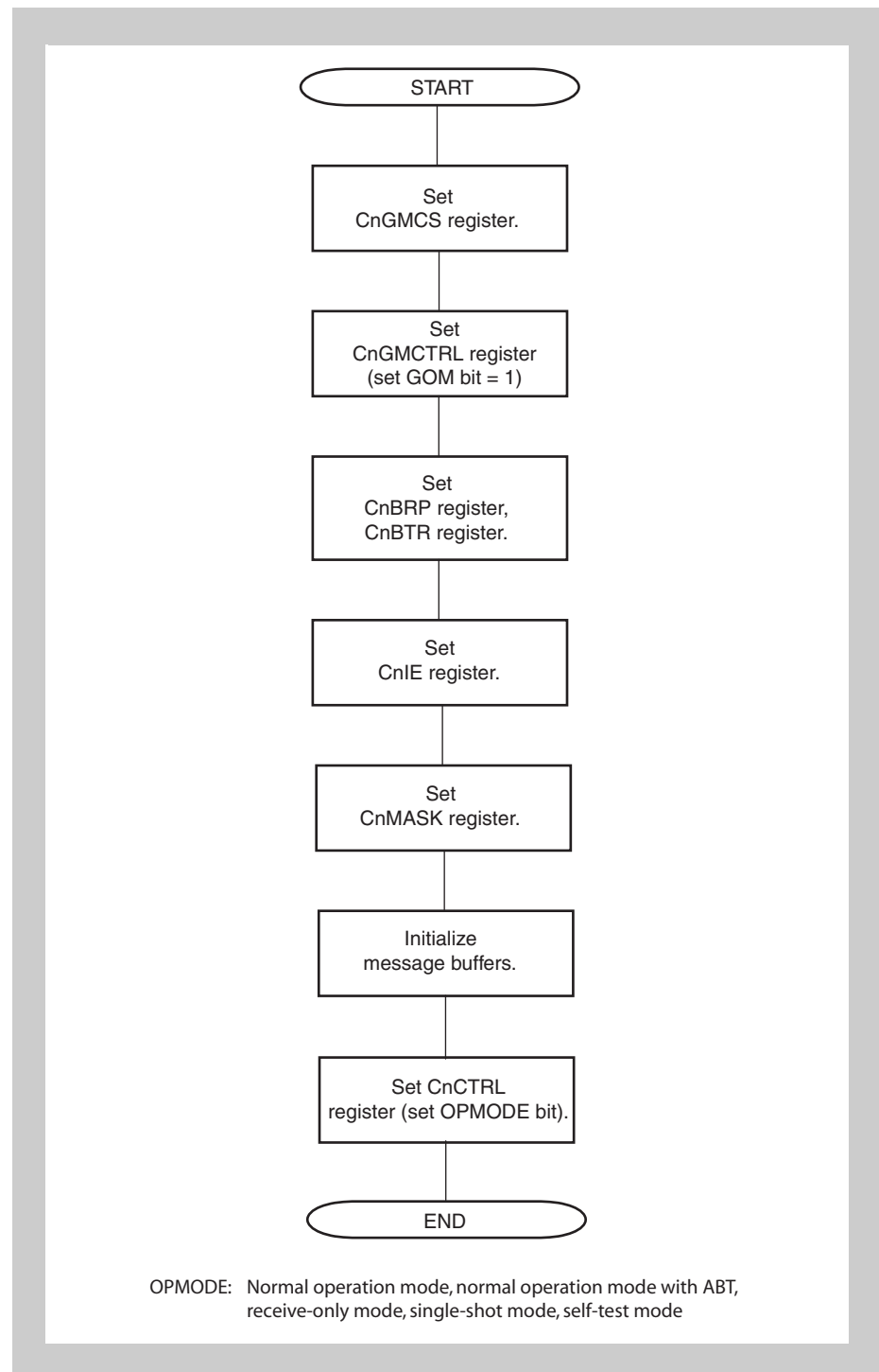
Figure 20-35 Initialization
