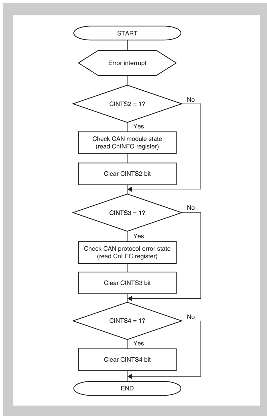
Figure 20-59 Error handling
