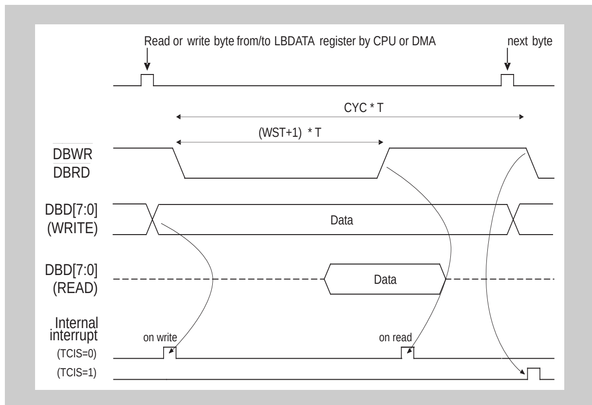
Figure 24-2 LCD Bus Interface timing (mod80 mode)
