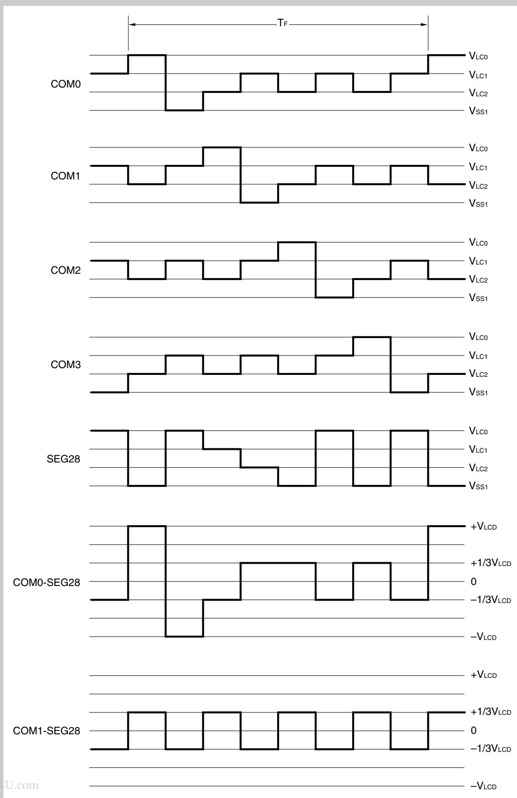
Figure 23-8 4-time-division LCD drive waveforms – examples
