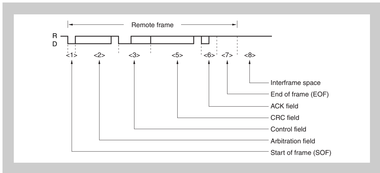
Figure 20-4 Remote frame
