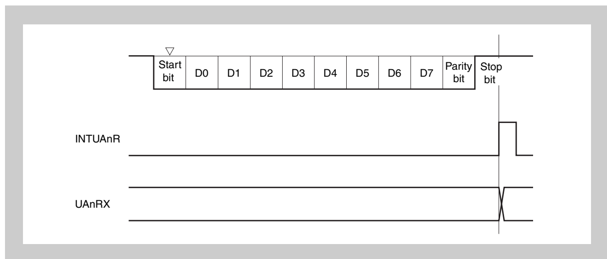
Figure 17-8 UART reception
