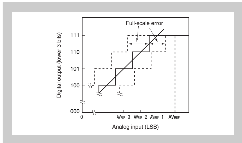
Figure 21-13 Full-scale error
