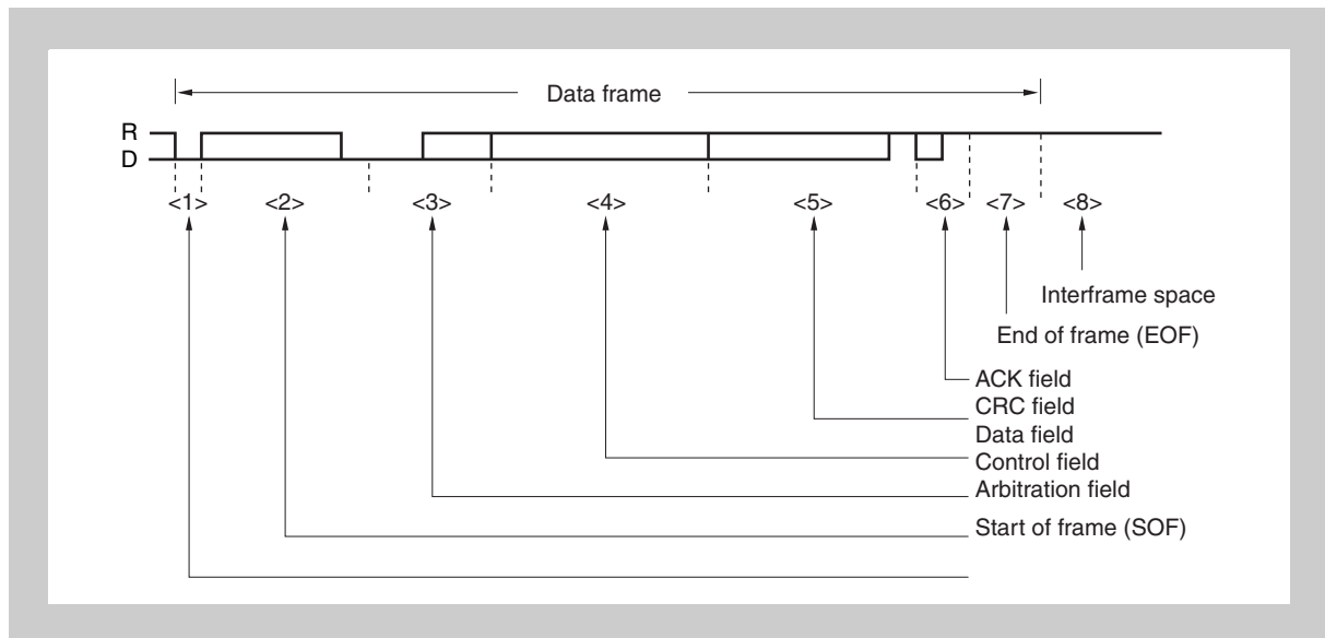
Figure 20-3 Data frame
