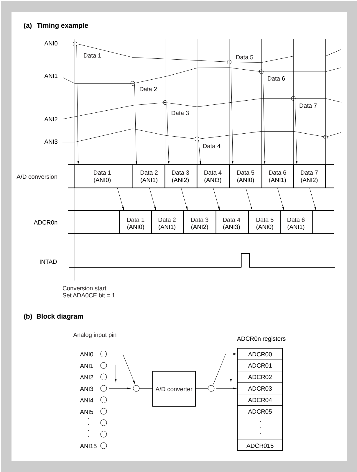
Figure 21-5 Timing example of continuous scan mode operation (ADA0S register = 03 H )
