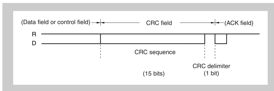
Figure 20-10 CRC field
