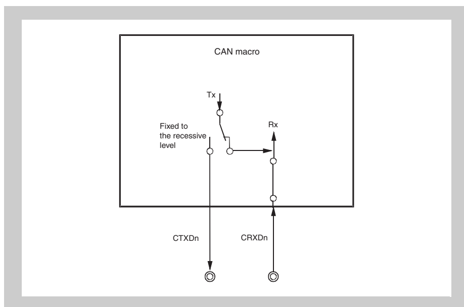
Figure 20-32 CAN module terminal connection in receive-only mode
