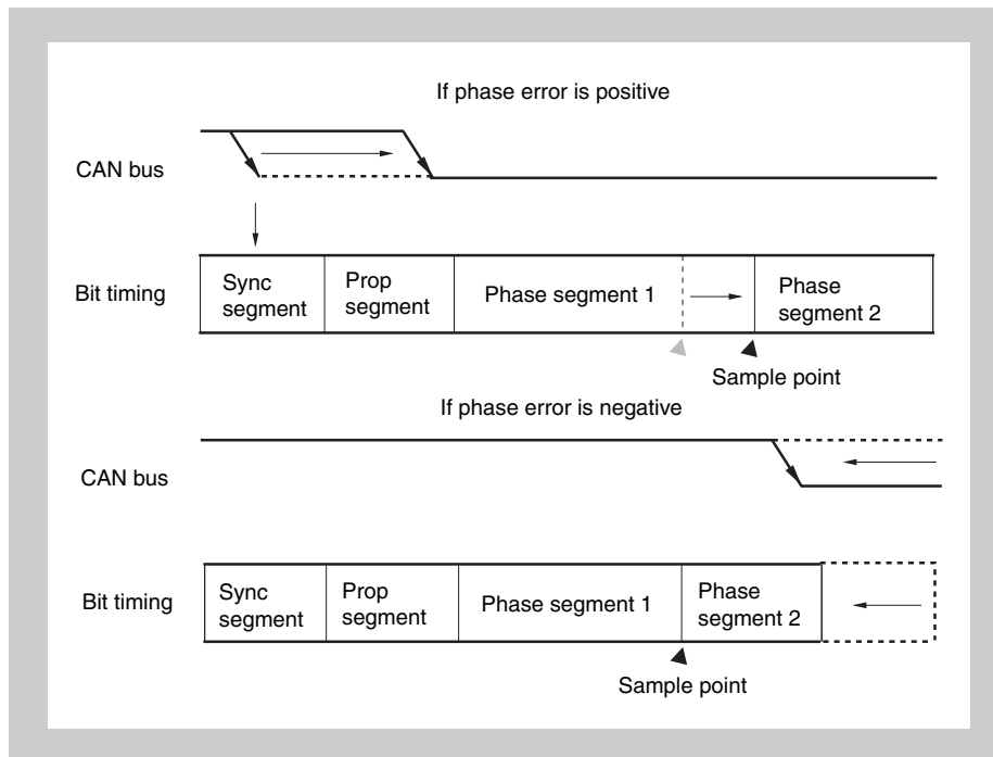
Figure 20-21 Resynchronization
