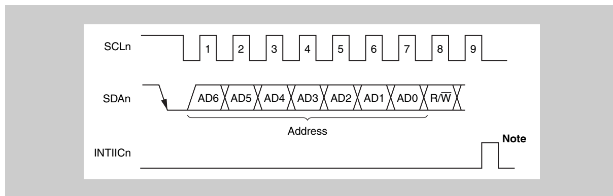
Figure 19-8 Address
