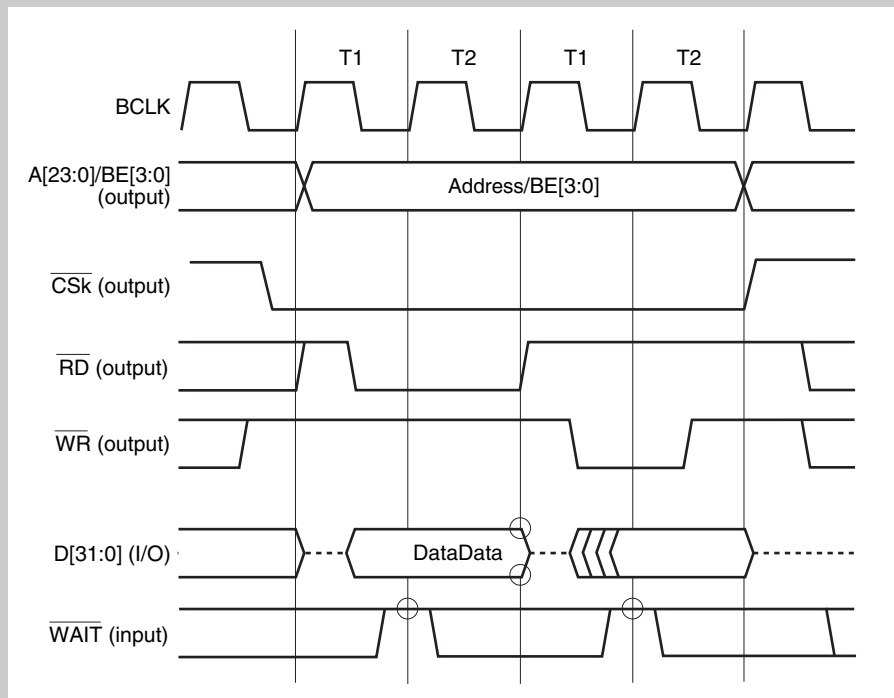
Figure 7-15 Read-write operation
