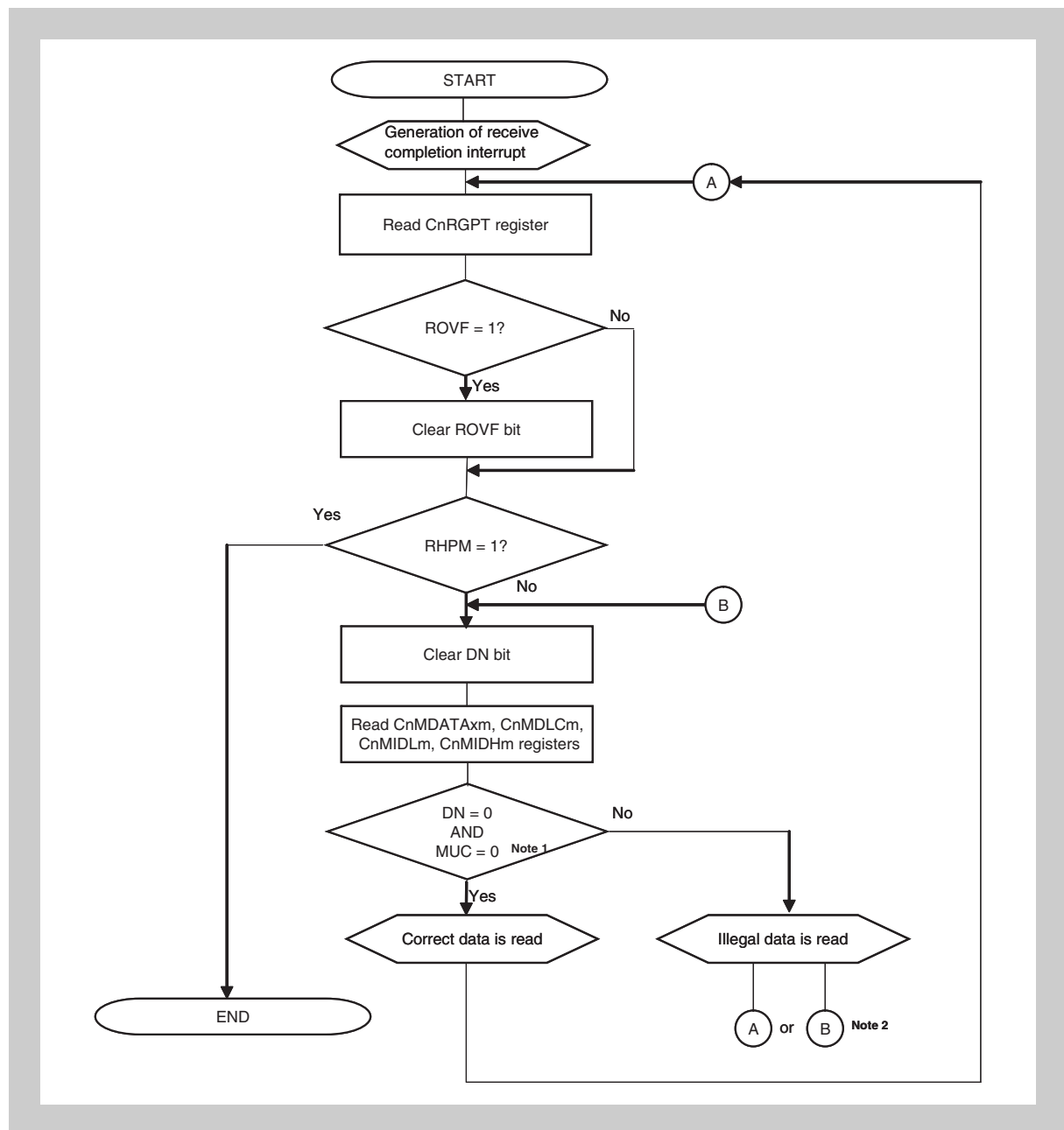
Figure 20-50 Reception via interrupt (using CnRGPT register)
