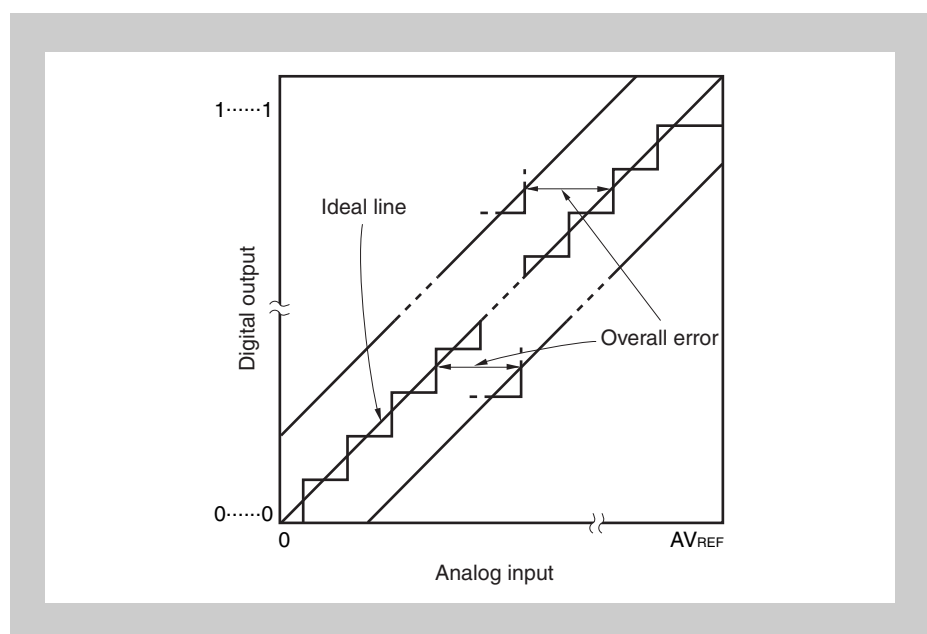
Figure 21-10 Overall error
