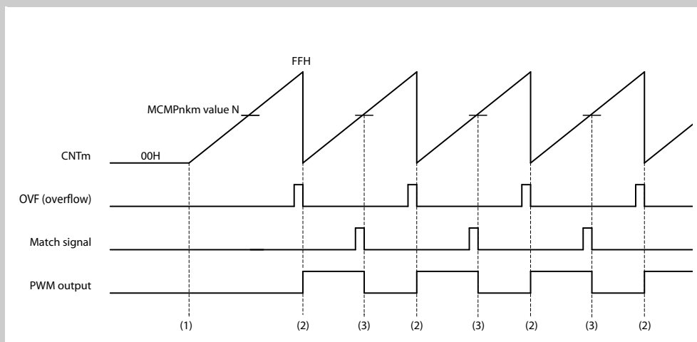
Figure 22-3 Output timing without 1-bit addition
