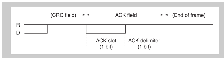
Figure 20-11 ACK field
