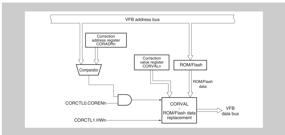
Figure 9-1 “Data Replacement” ROM correction block diagram
