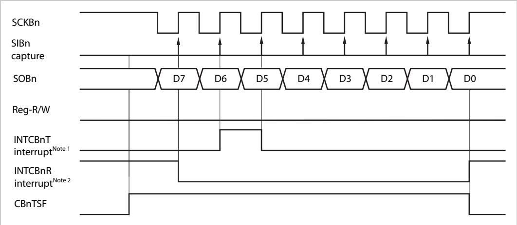
Figure 18-5 (i) Communication type 1 (CBnCKP = 0, CBnDAP = 0)
