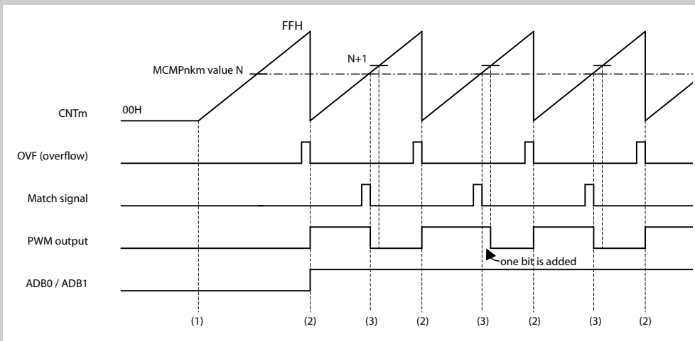
Figure 22-4 Output timing with 1-bit addition
