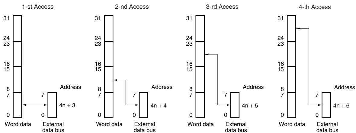
Figure 7-28 Access to address 4n + 3
