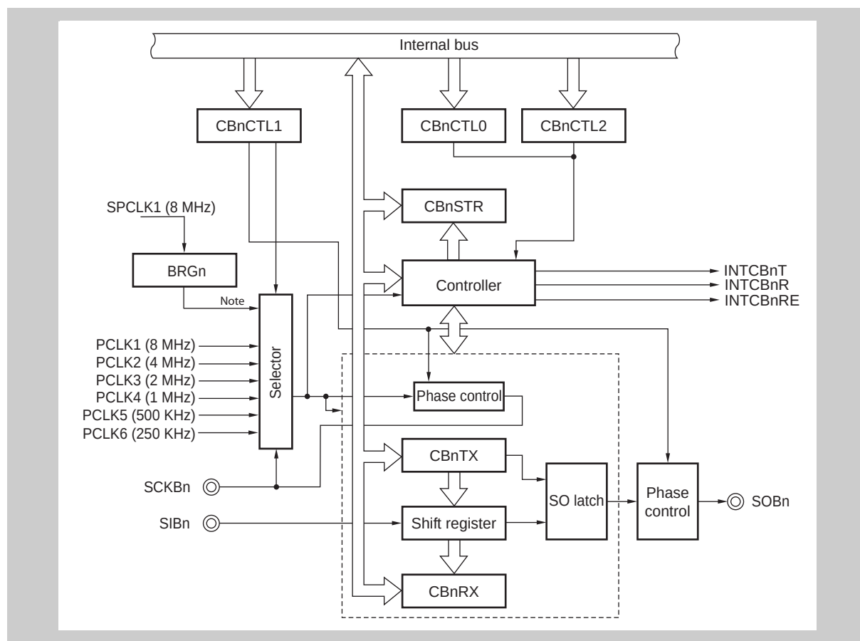
Figure 18-1 Block diagram of CSIBn
