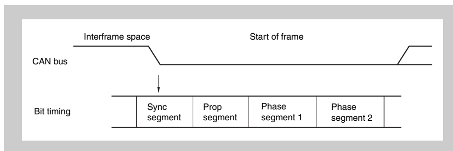
Figure 20-20 Adjusting synchronization of data bit
