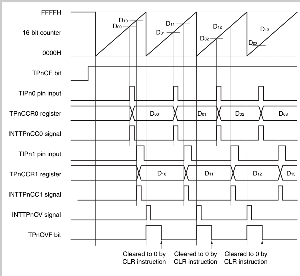
Figure 11-27 Basic timing in free-running timer mode (capture function)
