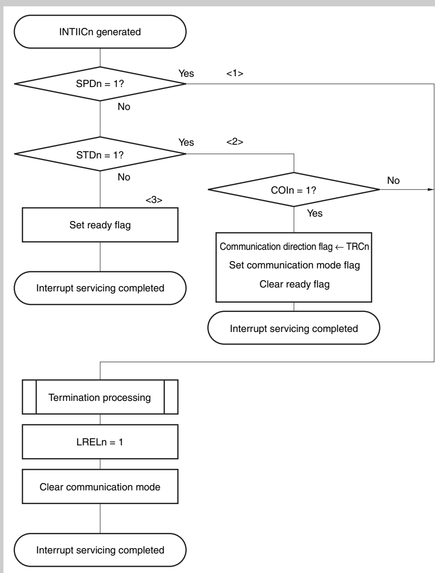
Figure 19-22 Slave operation flowchart (2)
