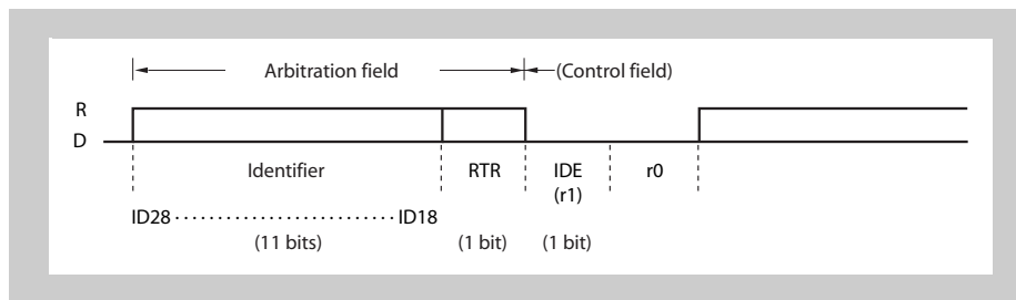
Figure 20-6 Arbitration field (in standard format mode)
