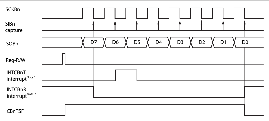
Figure 18-6 (ii) Communication type 3 (CBnCKP = 1, CBnDAP = 0)
