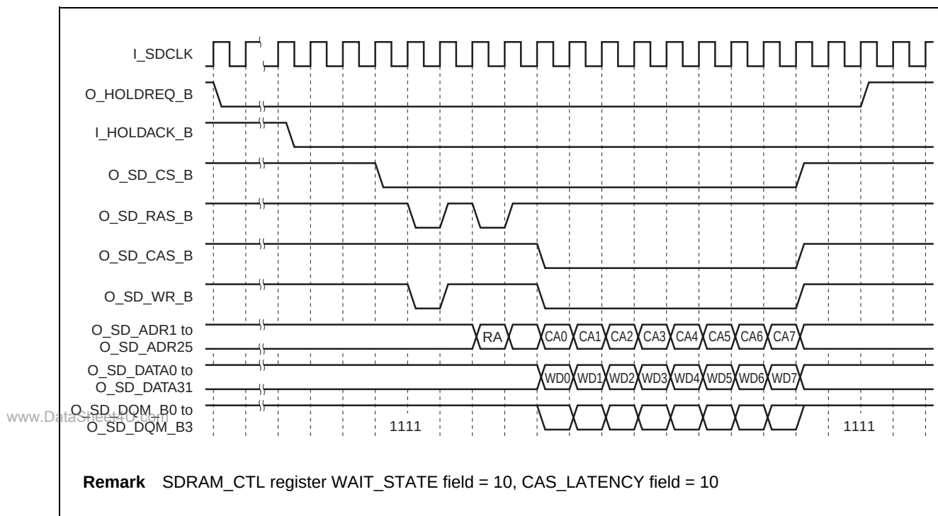
Figure 3-9. Main Memory (SDRAM) Write Access (8-Burst)
