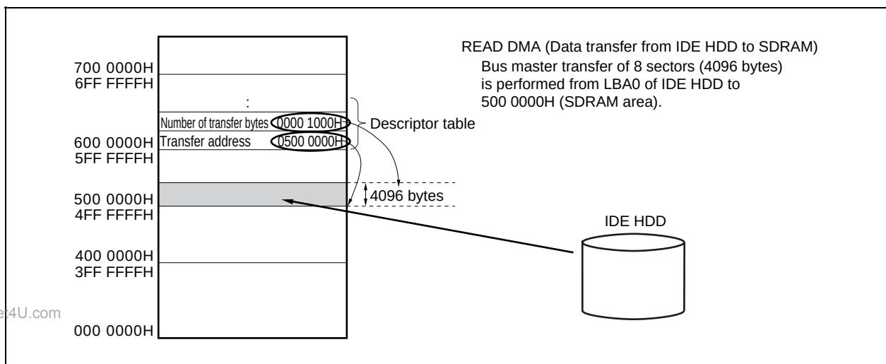
Figure 5-7. IDE_Read_DMA Function
