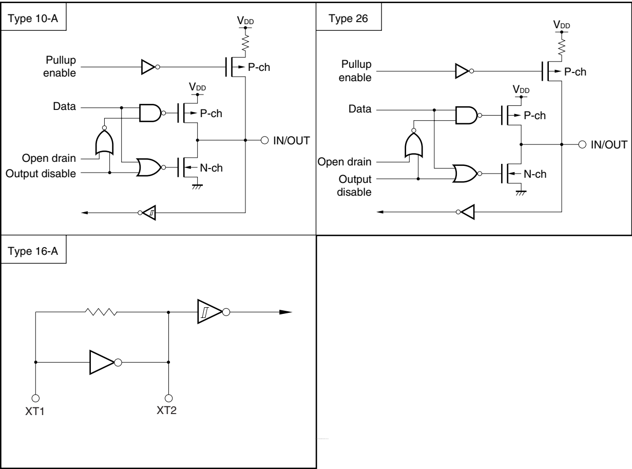
Figure 1-1. Pin Input/Output Circuits (2/2)
