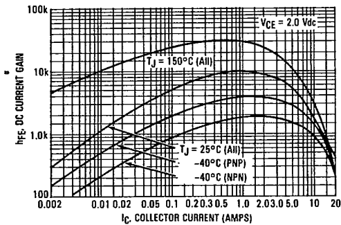
FIGURE 1 — TYPICAL DC CURRENT GAIN
