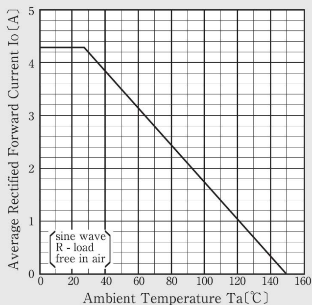
Derating Curve
