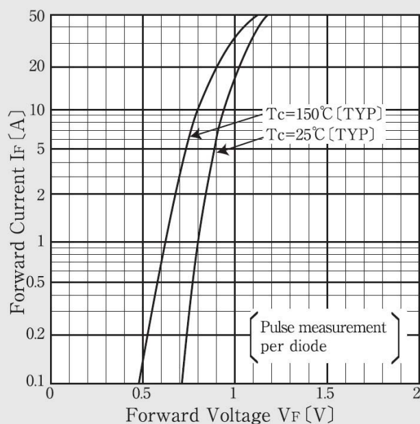
Forward Voltage
