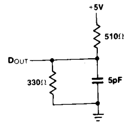
tLZ, tHZ LOAD CIRCUIT
