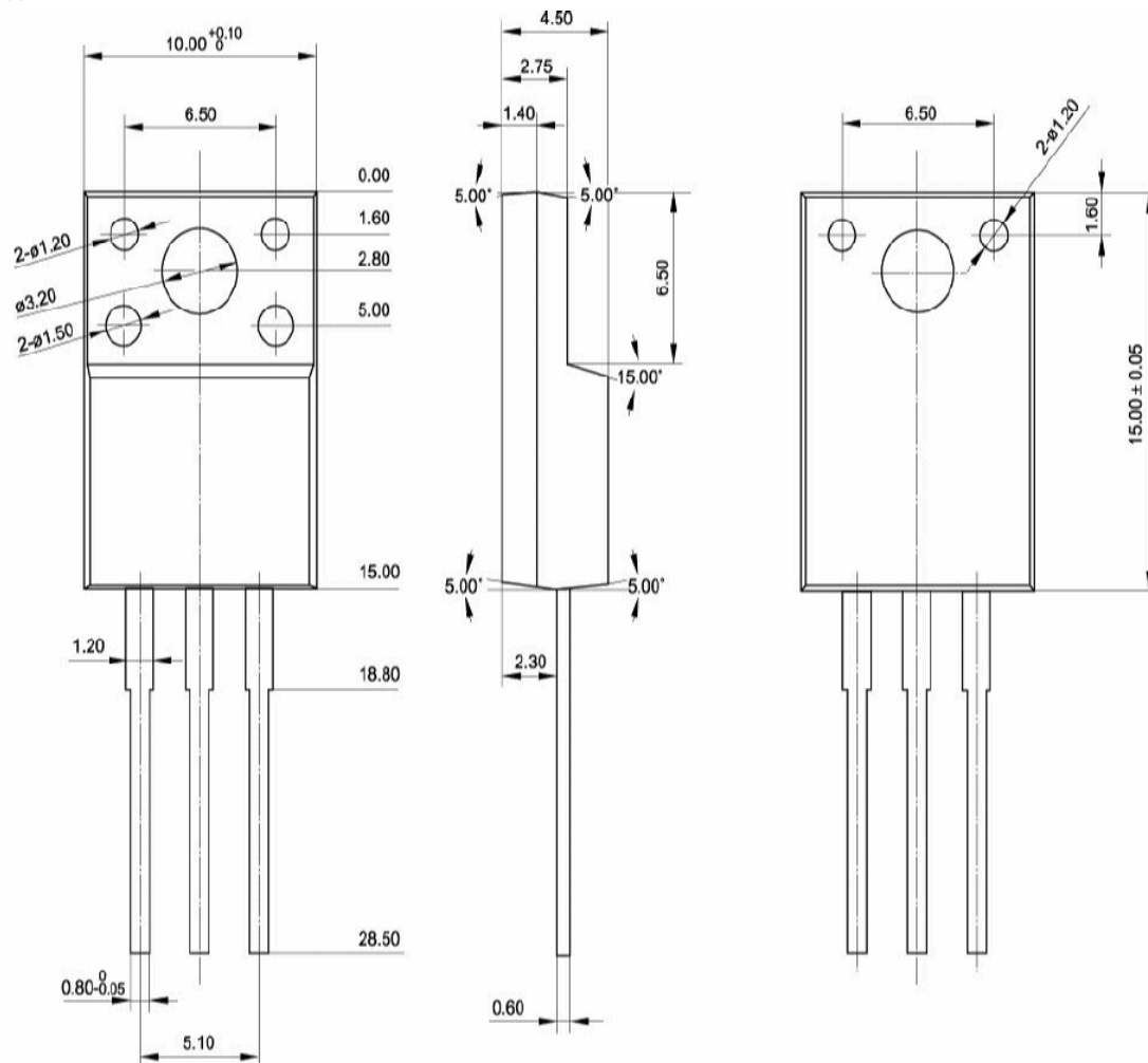
Fig.2 Outline dimensions
