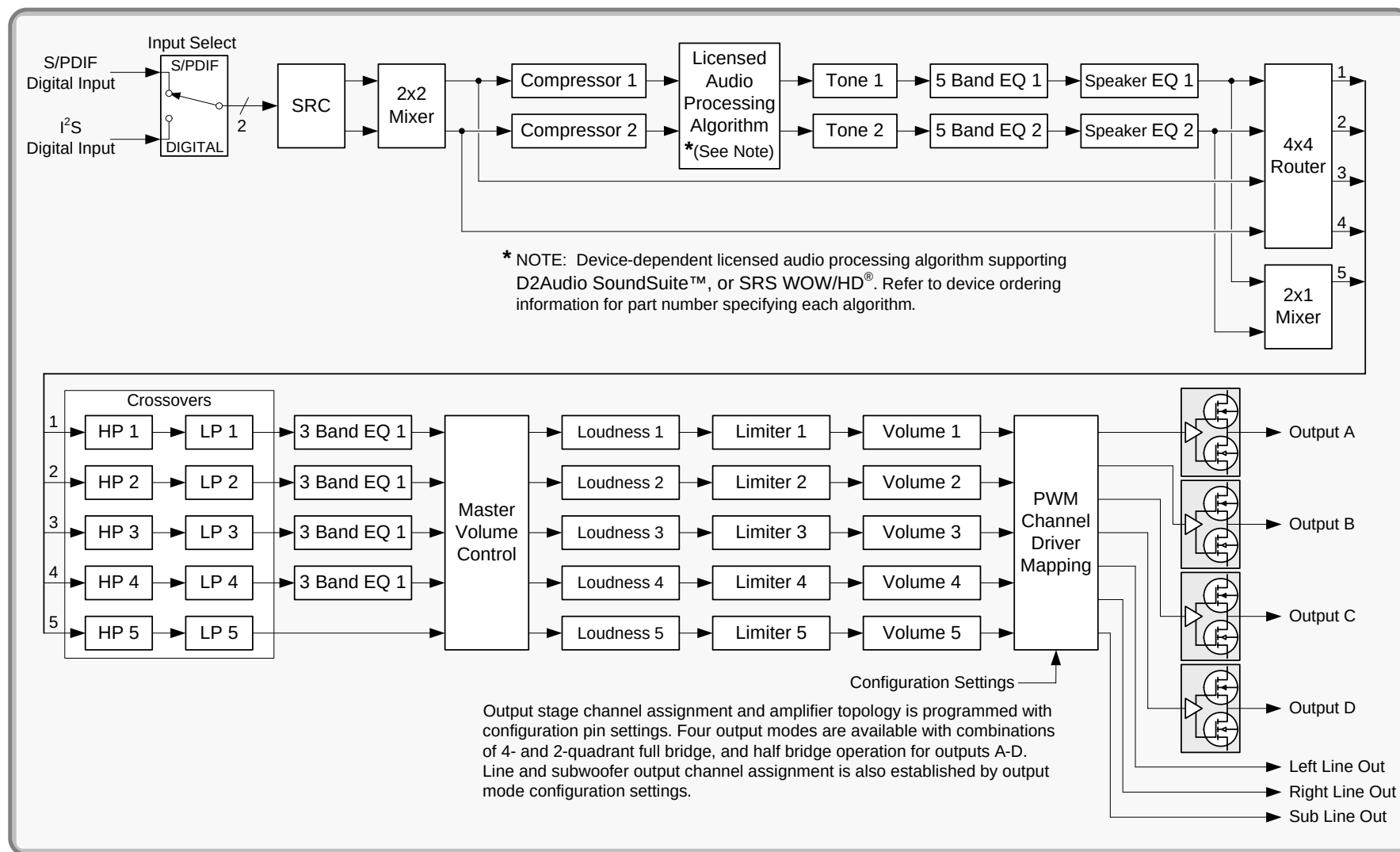
FIGURE 17. D2-45057, D2-45157 AUDIO SIGNAL FLOW
