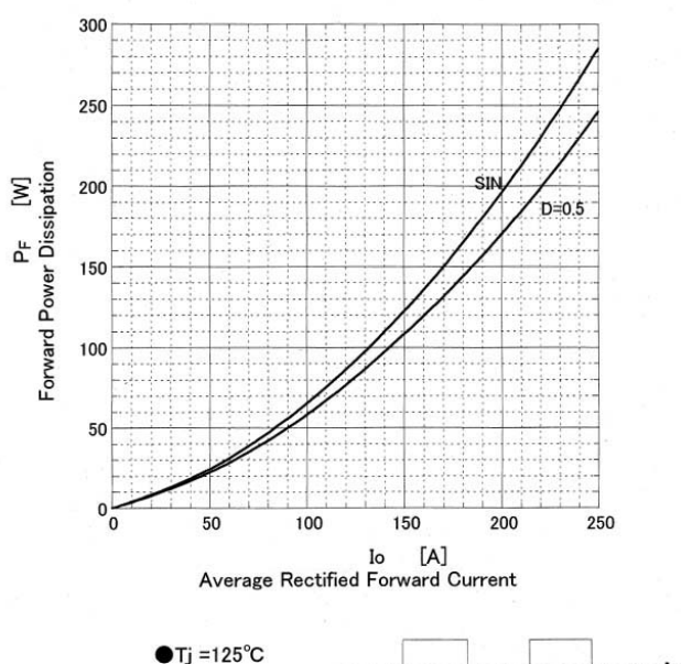
D180SC4M Forward Power Dissipation
