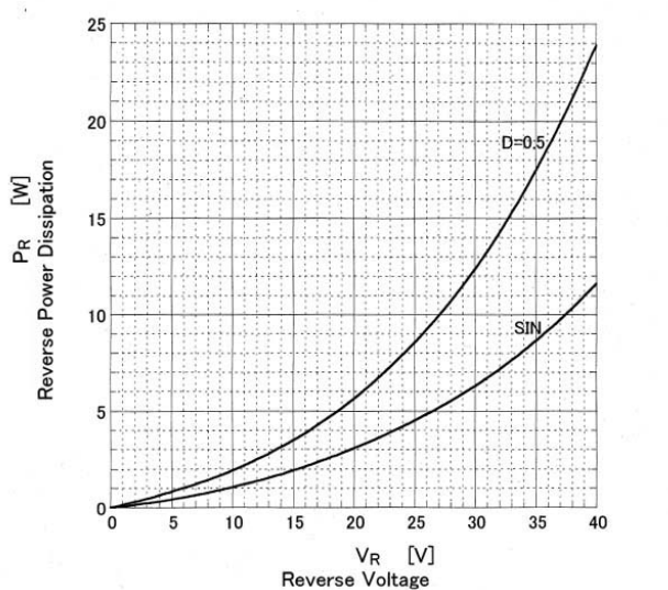
D180SC4M Reverse Power Dissipation
