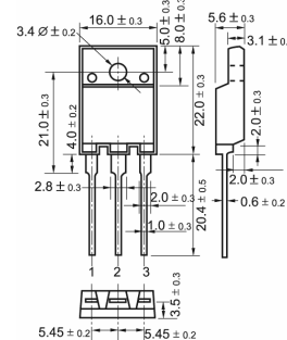
TO-3PML
