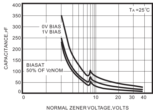
Fig.6 TYPICAL CAPACITANCE
