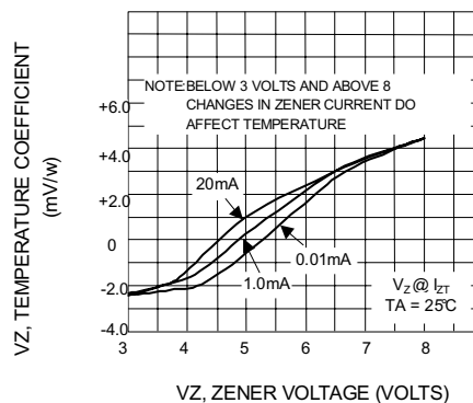
Fig. 4-EFFECT OF ZENER CURRENT
