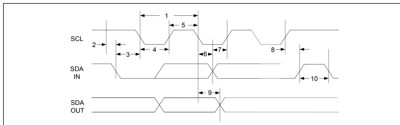
Figure 16. BSC Interface Timing Diagram
