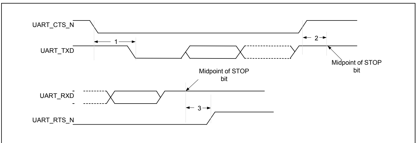
Figure 11. UART Timing
