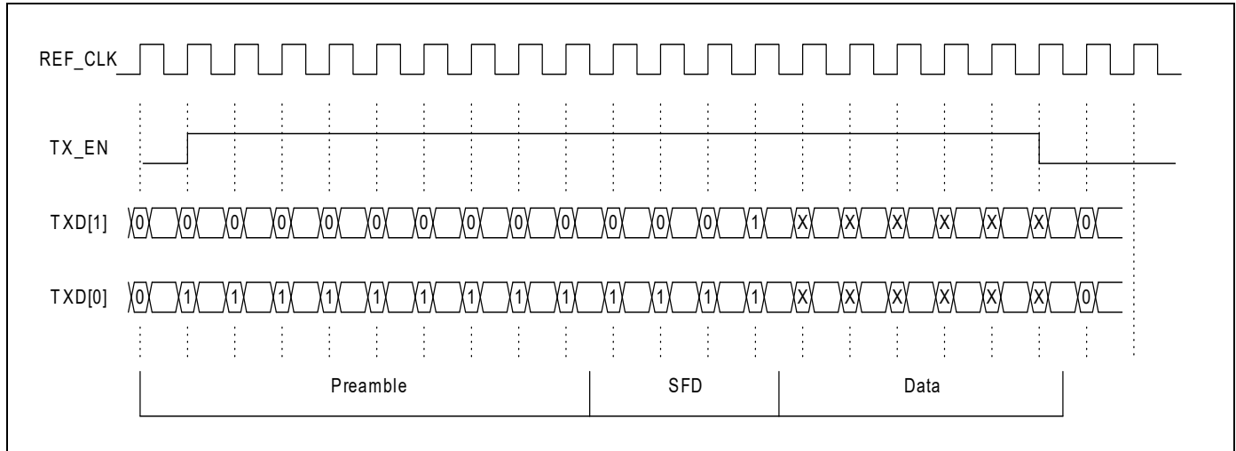
Figure 18. RMII Transmit Packet Timing
