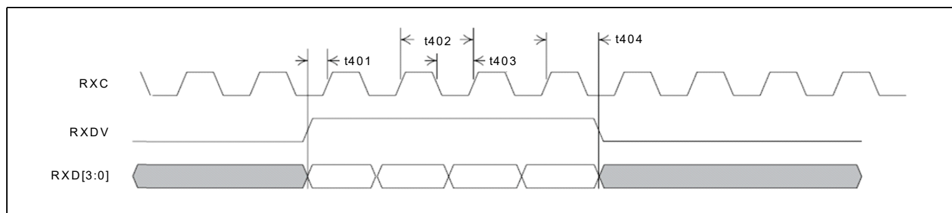
Figure 15. MII Receive Packet Timing
