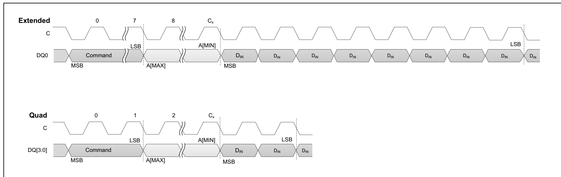
Figure 32. Memory-Write Timing
