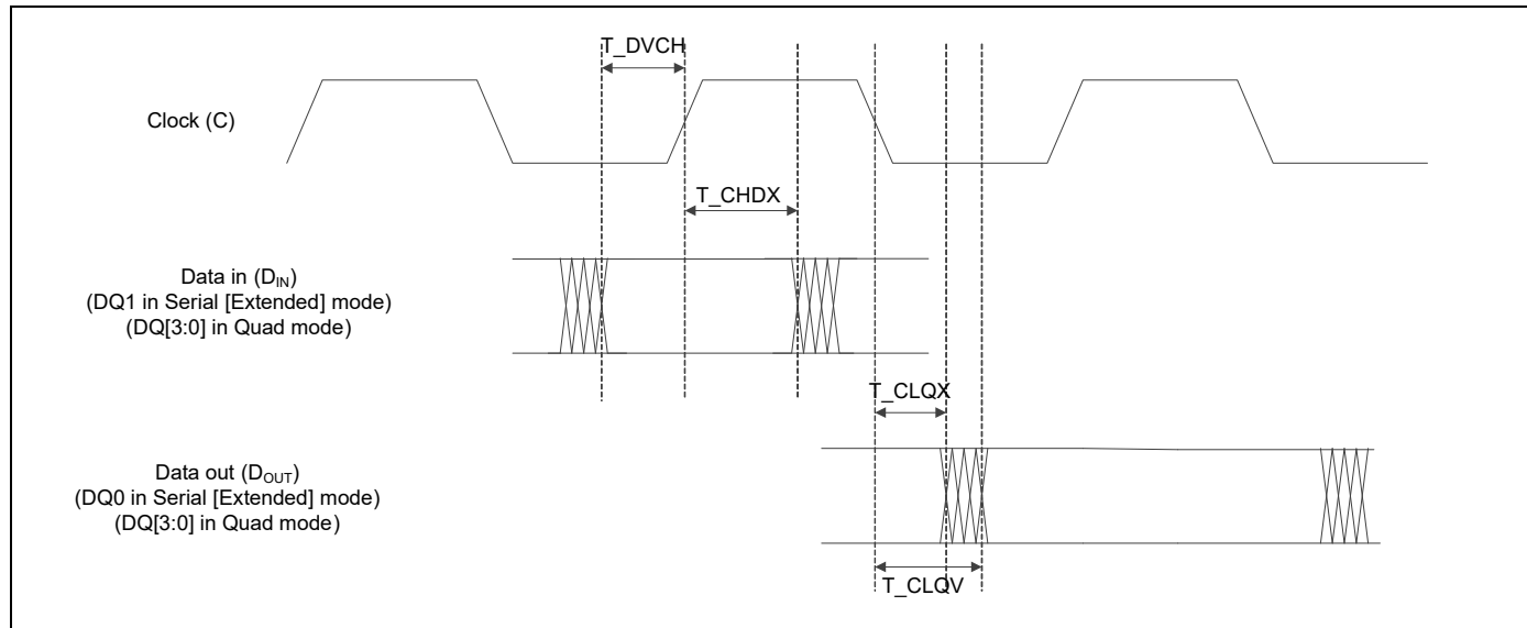
Figure 33. SPI Flash Timing Parameters Diagram
