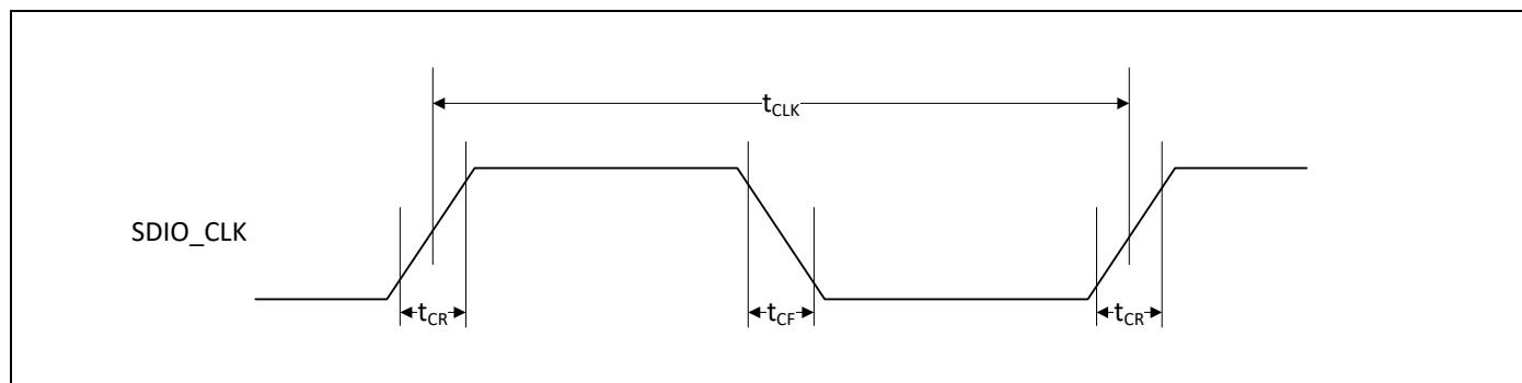
Figure 24. SDIO Clock Timing (SDR Modes)
