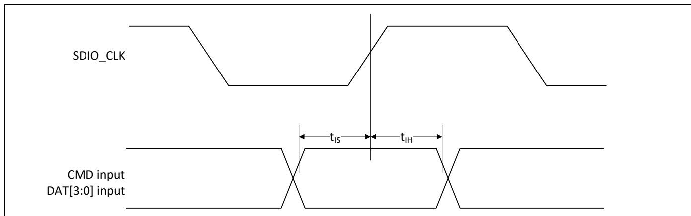
Figure 25. SDIO Bus Input Timing (SDR Modes)
