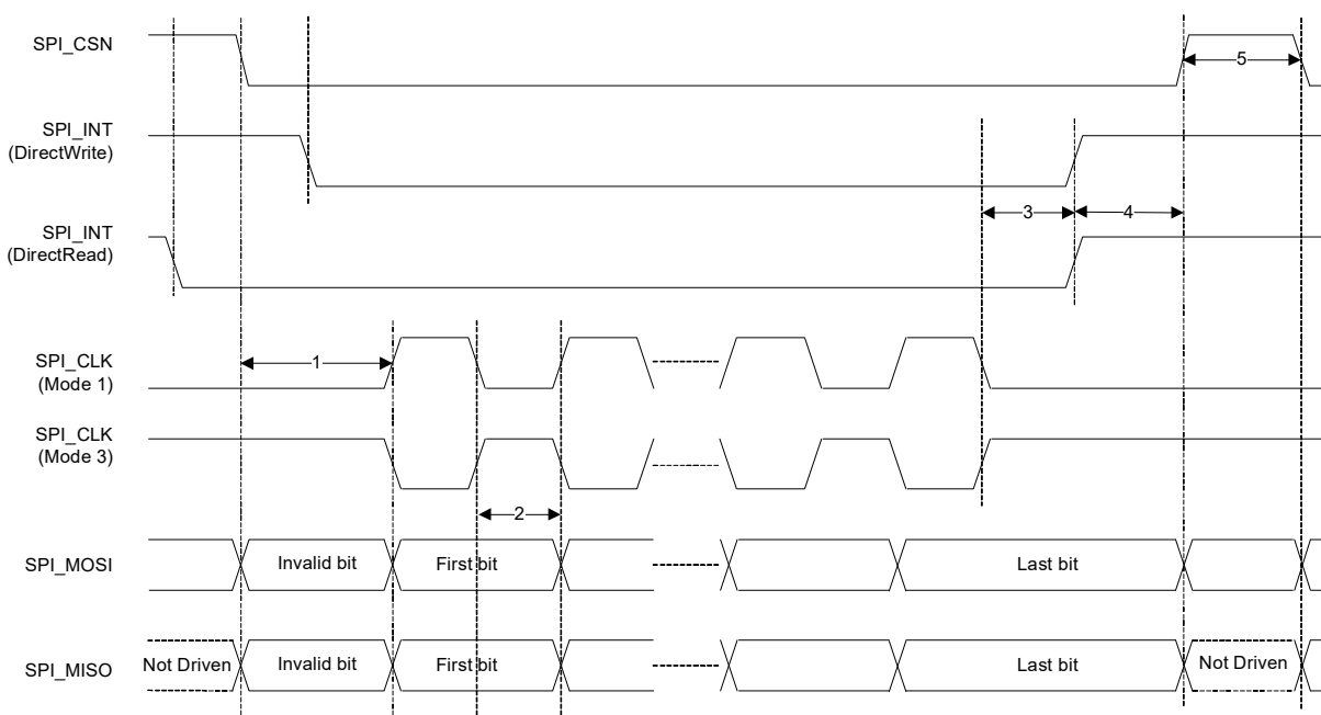
Figure 10. SPI Timing, Mode 1 and 3
