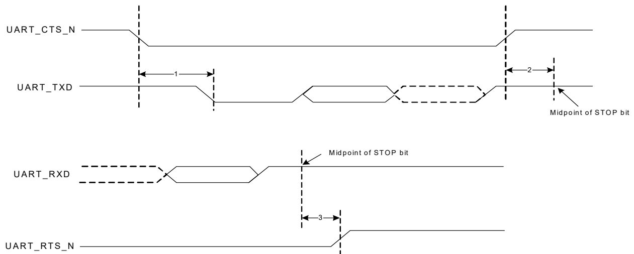
Figure 8. UART Timing
