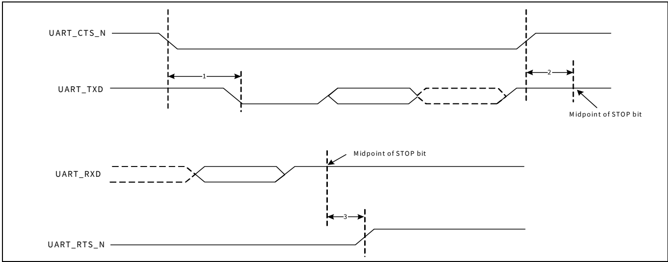
Figure 8 UART timing
