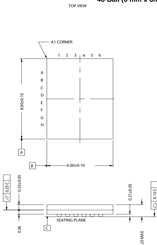
48-Ball (6 mm x 8mm x 1.2 mm) FBGA BA48K
