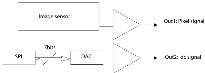
Figure 7. Output Stage Architecture.
