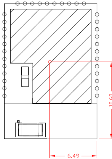
Figure 23. CYBT-4830xx-02 Center of Mass
