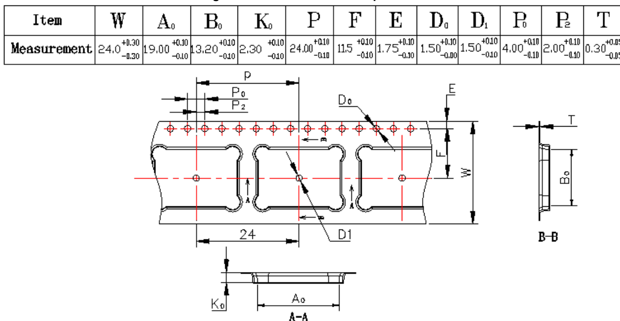
Figure 20. CYBT-4830xx-02 Tape Dimensions
