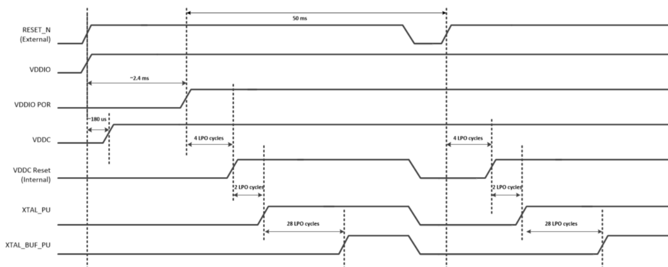
Figure 11. Reset Timing
