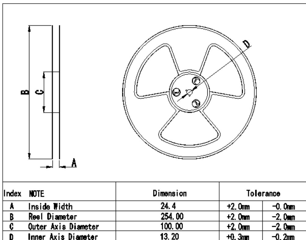
Figure 22. Reel Dimensions
