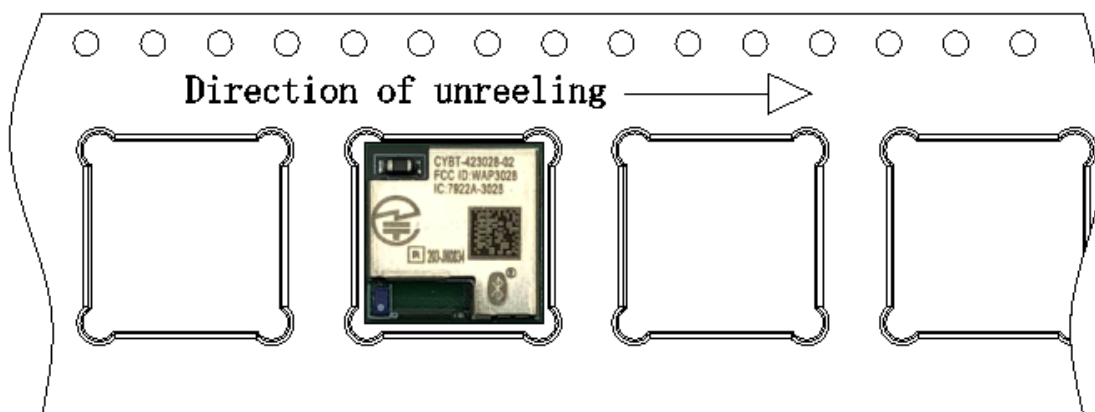
Figure 21. Component Orientation in Tape and Unreeling Direction
