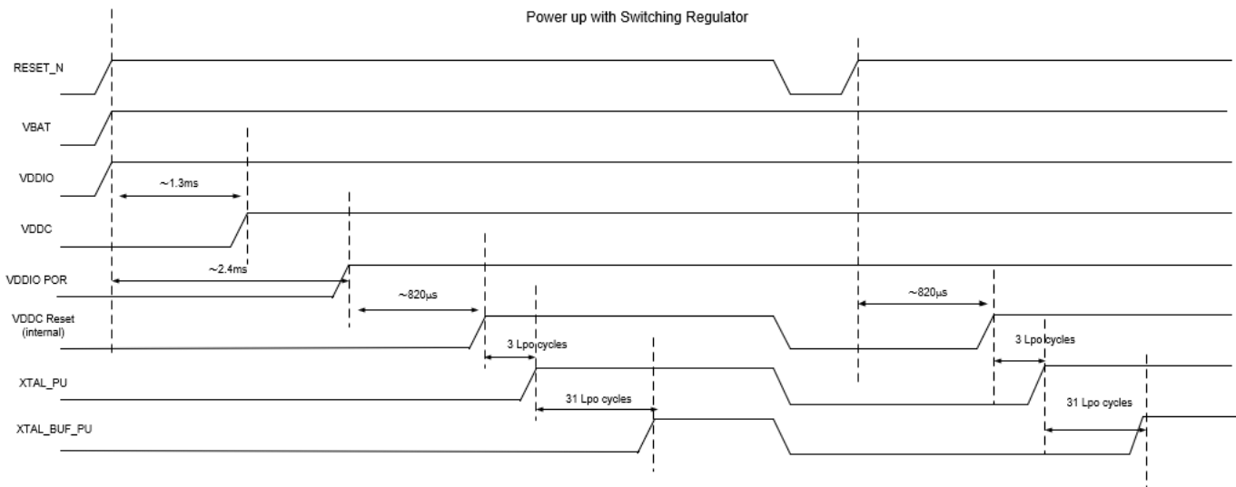
Figure 10. Reset Timing
