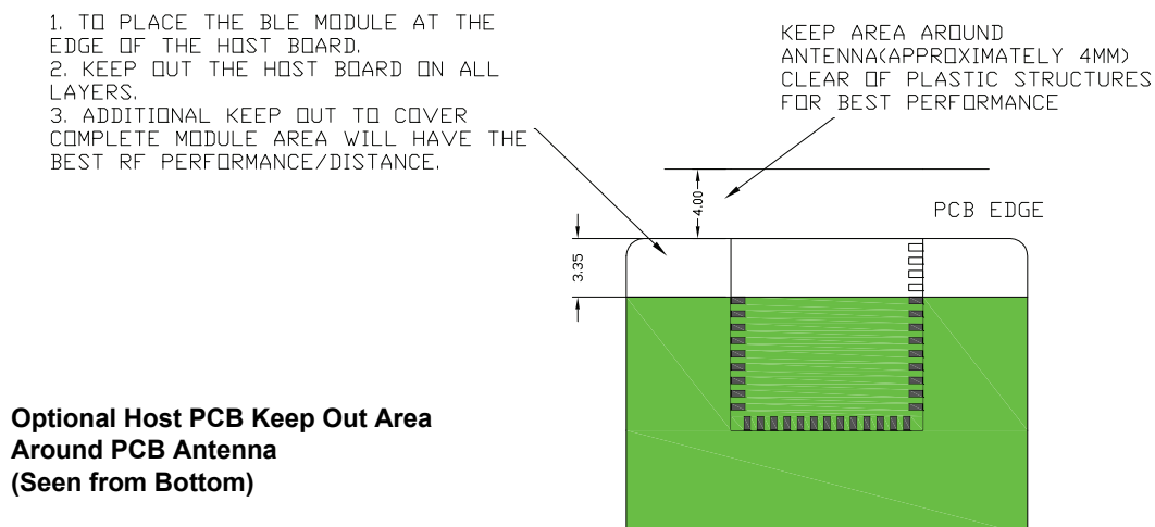
Figure 4. Optional Additional Host PCB Keep Out Area Around the CYBT-2x305x-02 PCB Antenna
