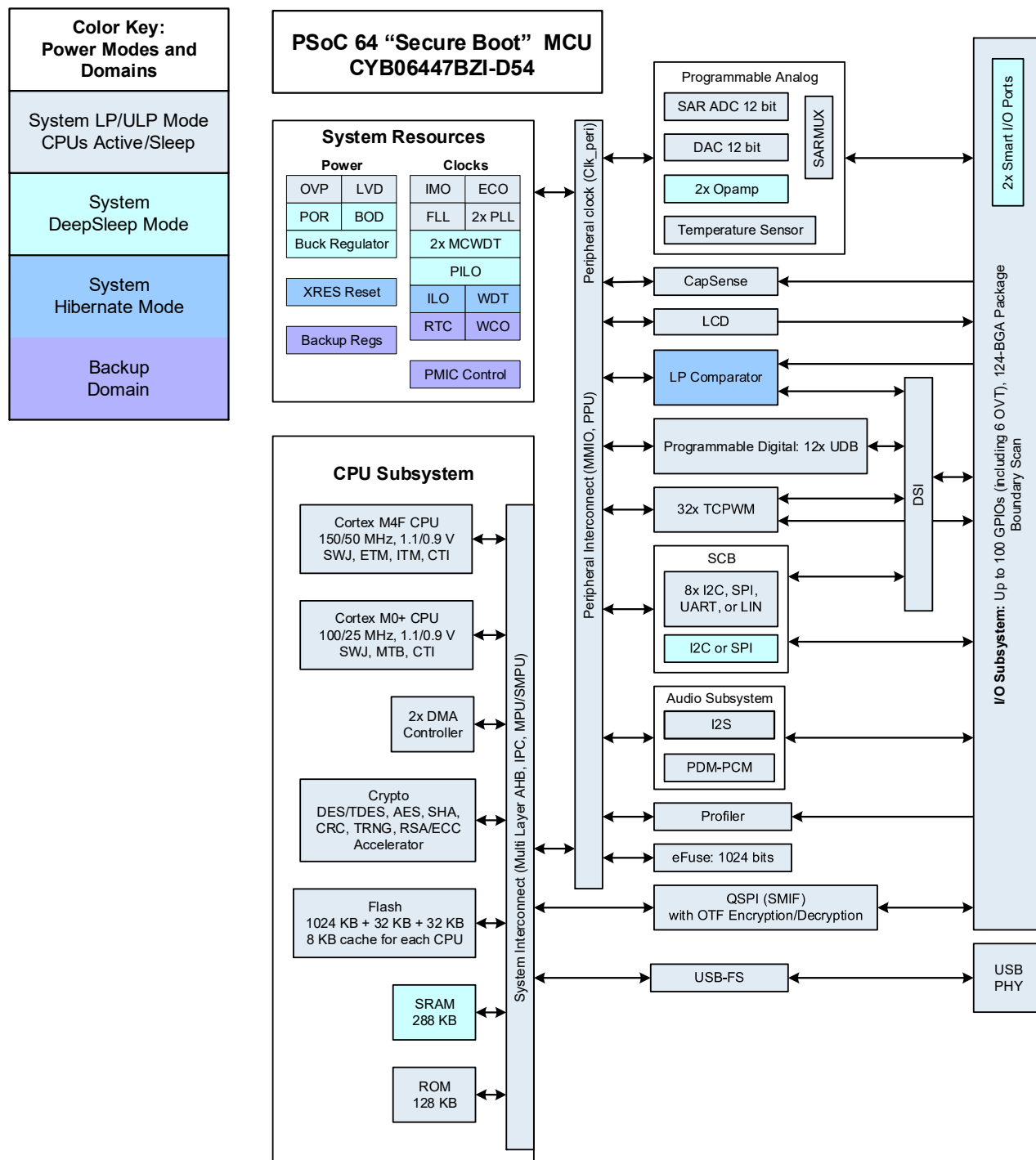
Figure 2. Block Diagram
