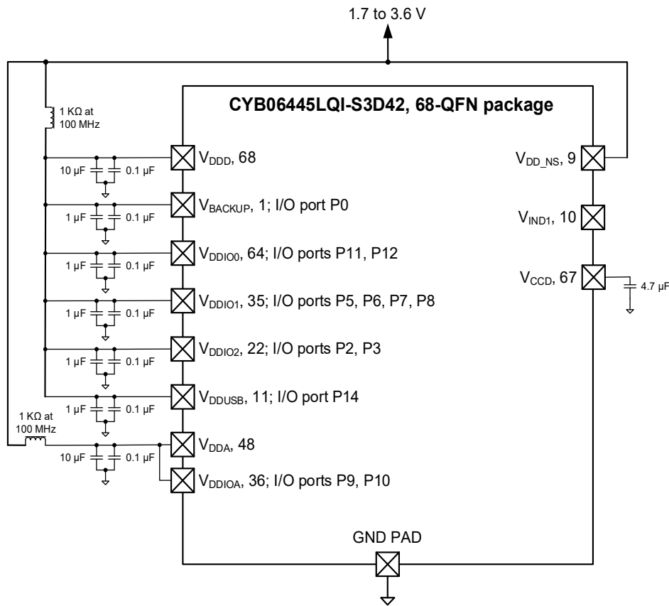
Figure 15. 68-QFN (No Buck) Power Connections Diagram
