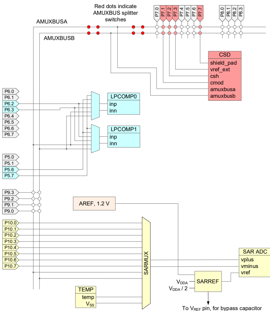
Figure 6. Analog Subsystem
