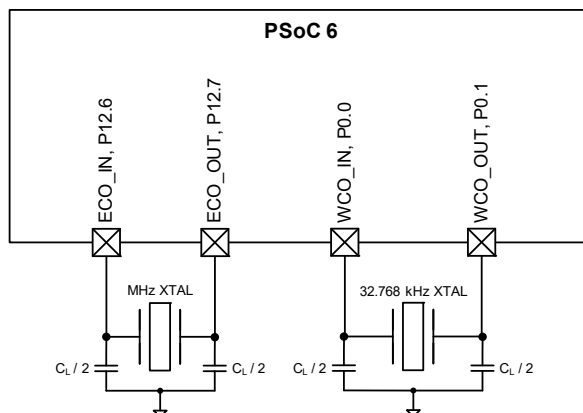
Figure 4. Oscillator Circuits
