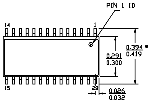
28-lead (300-mil) Molded SOIC S21
