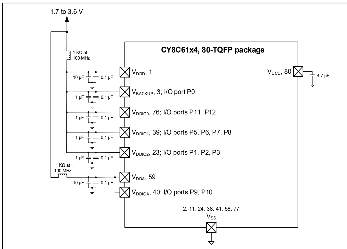
Figure 12 80-TQFP Power Connection Diagram
