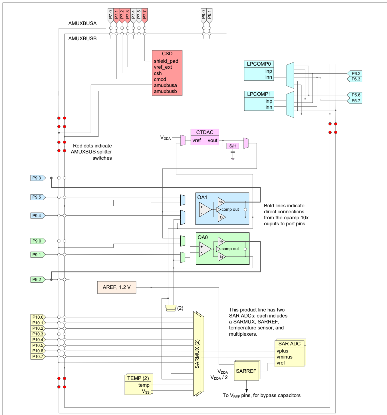
Figure 6 Analog subsystem
