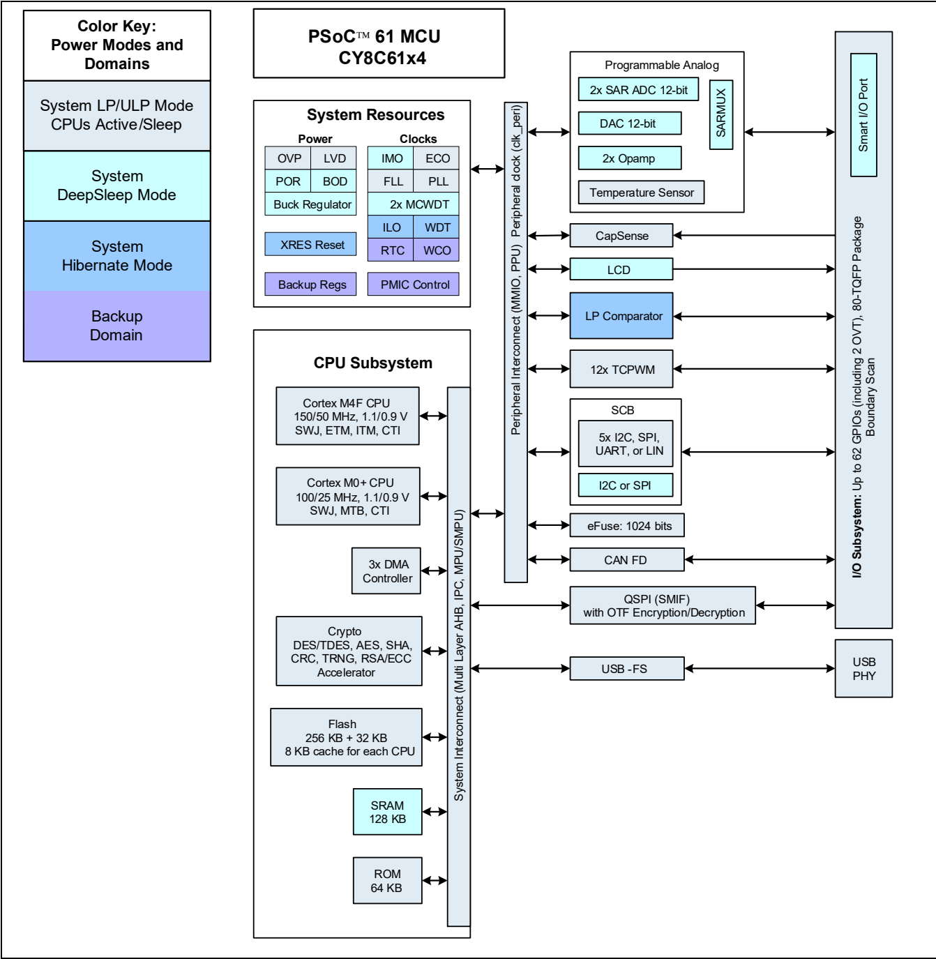
Figure 2 Block diagram
