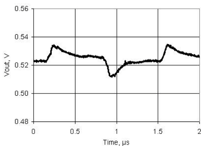
Figure 11-38. VDAC Glitch Response, Codes 0x7F - 0x80, 1 V Mode, Fast Mode, V dda = 5 V
