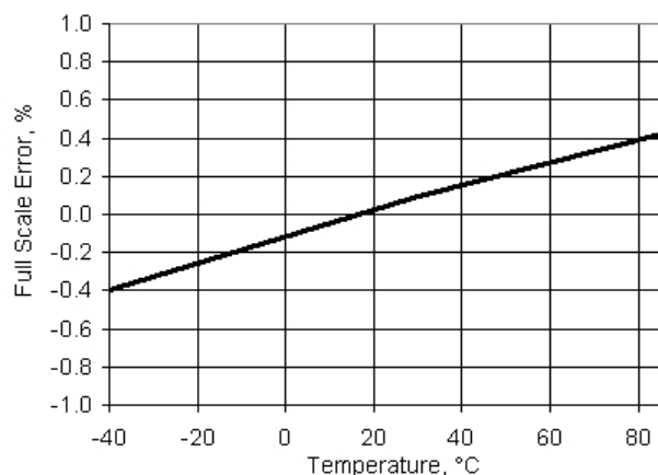
Figure 11-33. VDAC Full Scale Error vs Temperature, 1 V Mode
