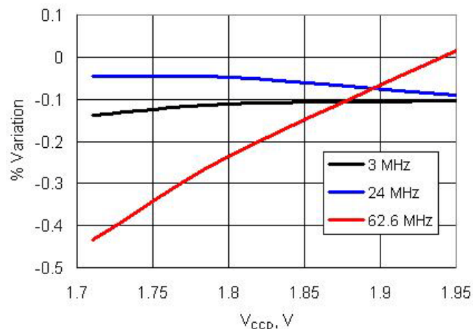
Figure 11-43. IMO Frequency Variation vs. V CCD
