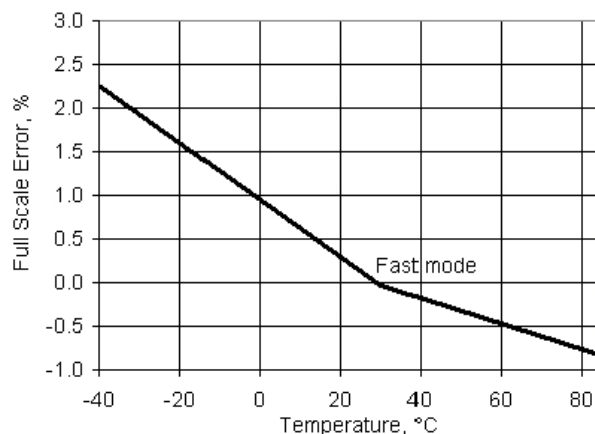
Figure 11-23. IDAC Full Scale Error vs Temperature, Range = 255 \mu A, Sink Mode
