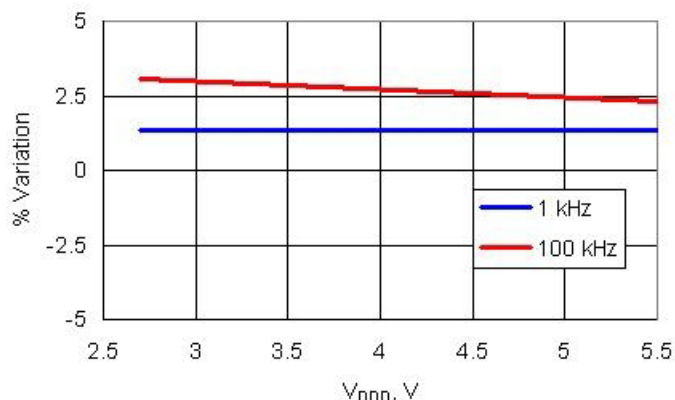
Figure 11-45. ILO Frequency Variation vs. V_{DD}
