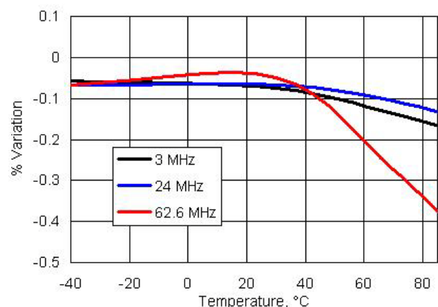
Figure 11-42. IMO Frequency Variation vs. Temperature
