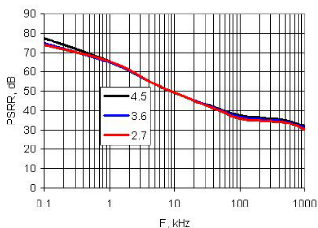
Figure 11-2. Digital Regulator PSRR vs Frequency and V_{DD}
