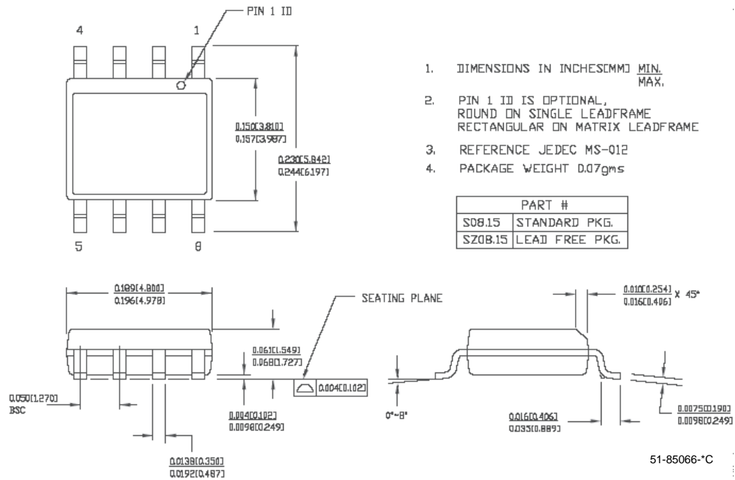
Figure 11-1. 8-Lead (150) SOIC
