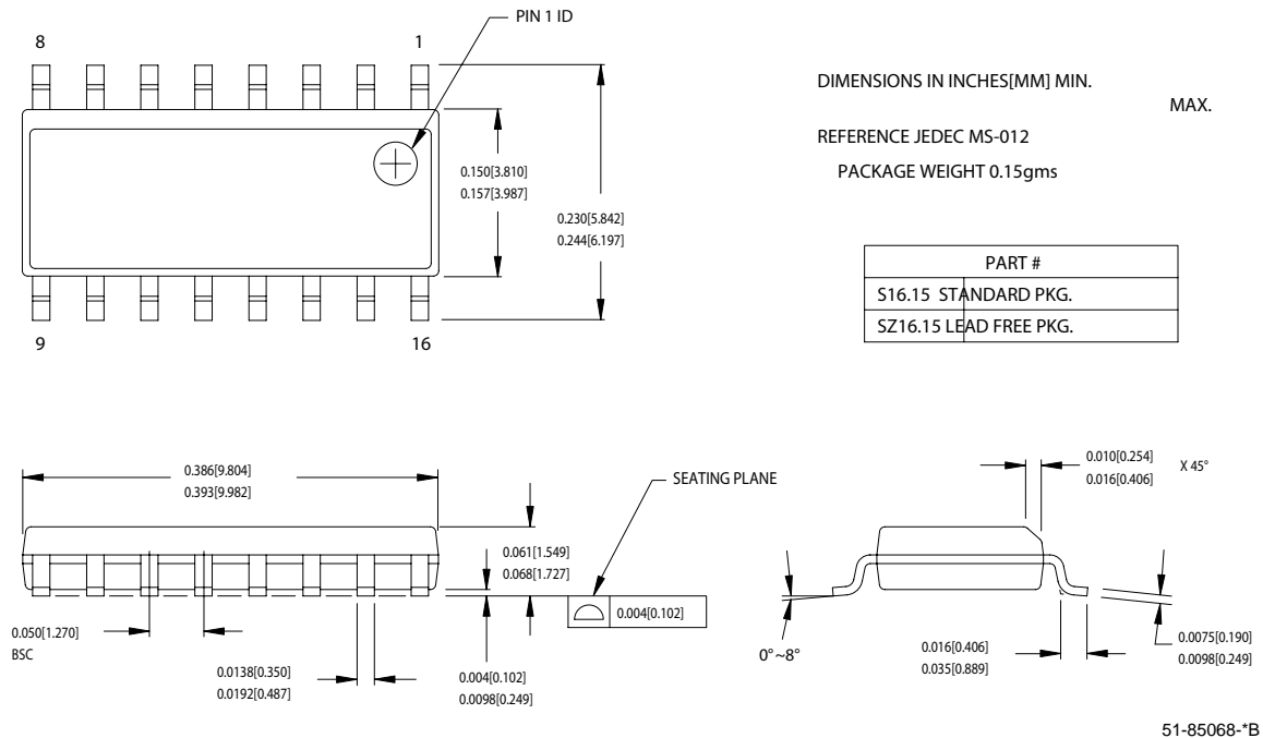
Figure 11-2. 16-Lead (150) SOIC
