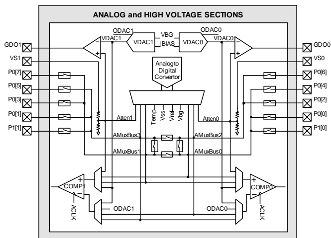
Figure 4-1. Analog Block Diagram
