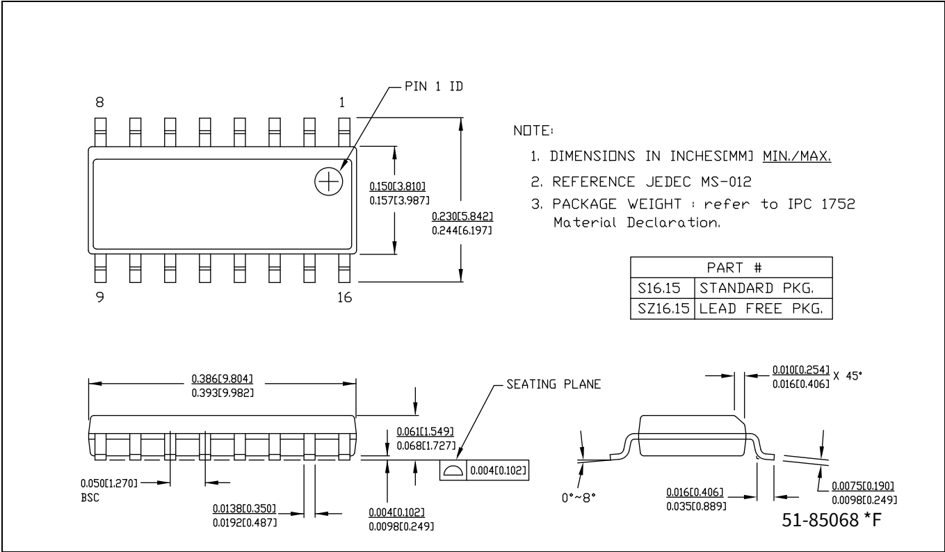
Figure 7 16-pin SOIC (150 Mils) package outline (PG-DSO-16)
