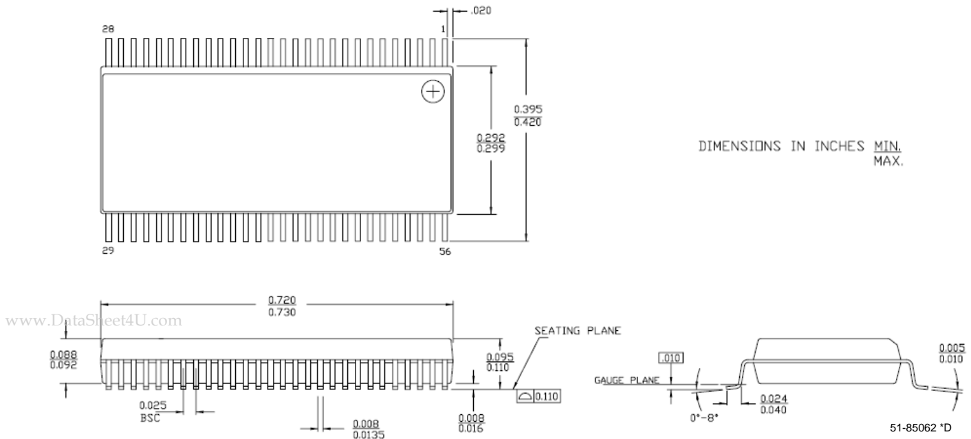
Figure 14. 56-Pin (300-Mil) SSOP
