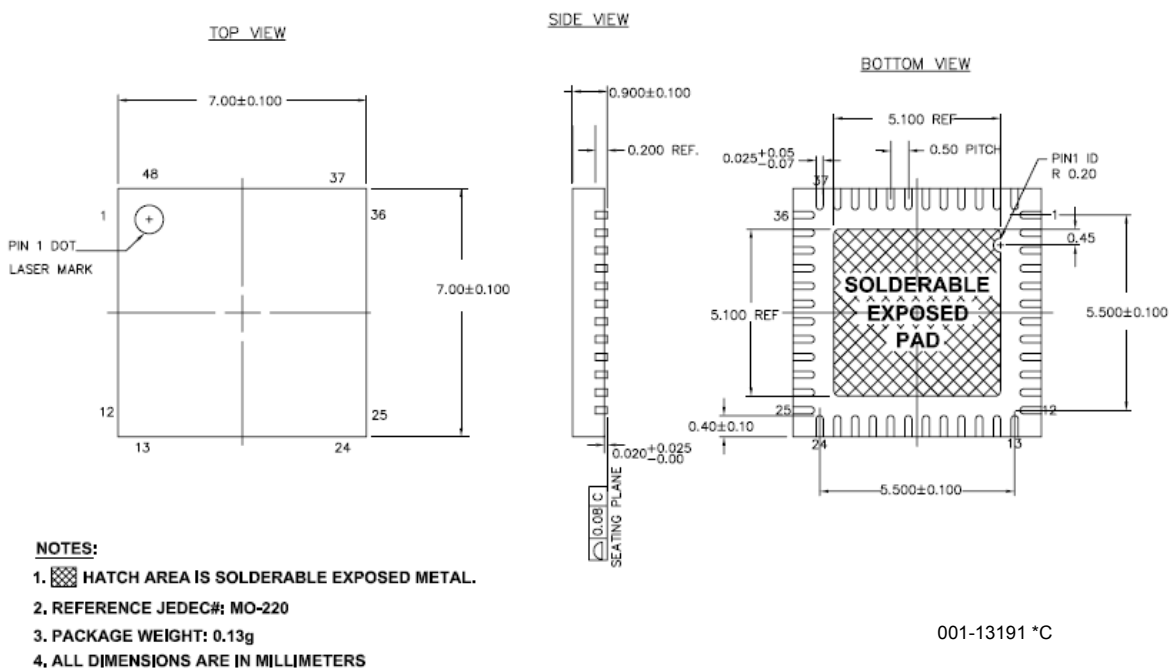
Figure 17. 48-Pin (7x7 mm) QFN
