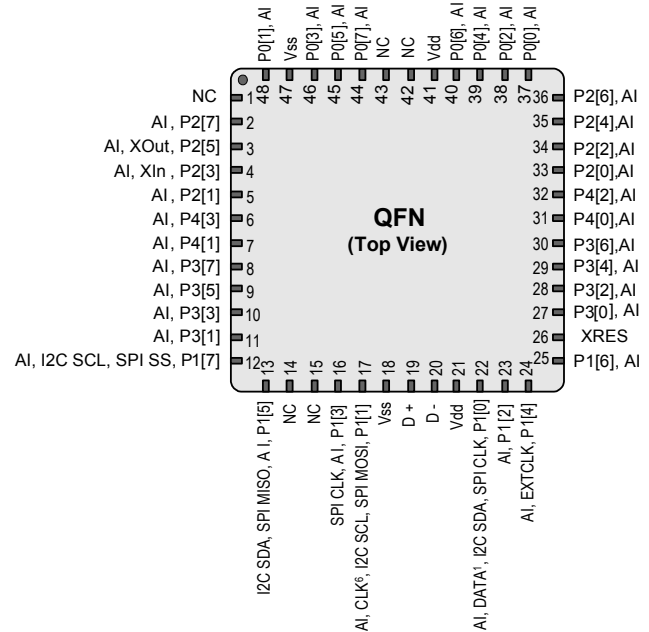
Figure 6. CY8C20666 48-Pin QFN PSoc Device
