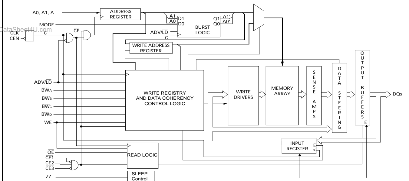
Logic Block Diagram—CY7C1379C (256K x 36)
