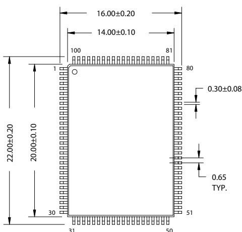
100-Pin Thin Plastic Quad Flatpack (14 x 20 x 1.4 mm) (51-85050)
