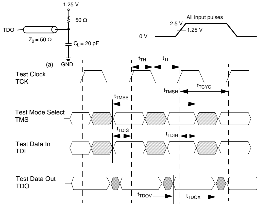
Figure 3. TAP Timing and Test Conditions
