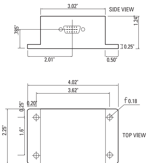
Aluminum Package
