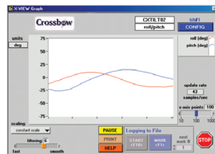
Figure 2. Development Software
