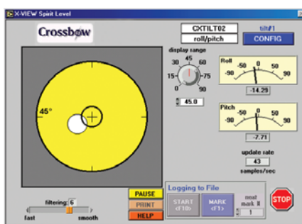
Figure 1. Development Software
